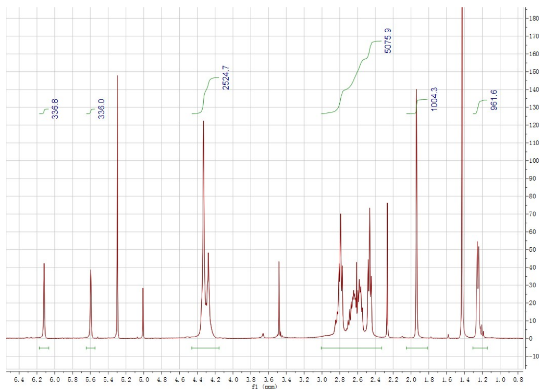
Figure S1. 1 H NMR spectrum of G4 dendrimer in DCCl 3
