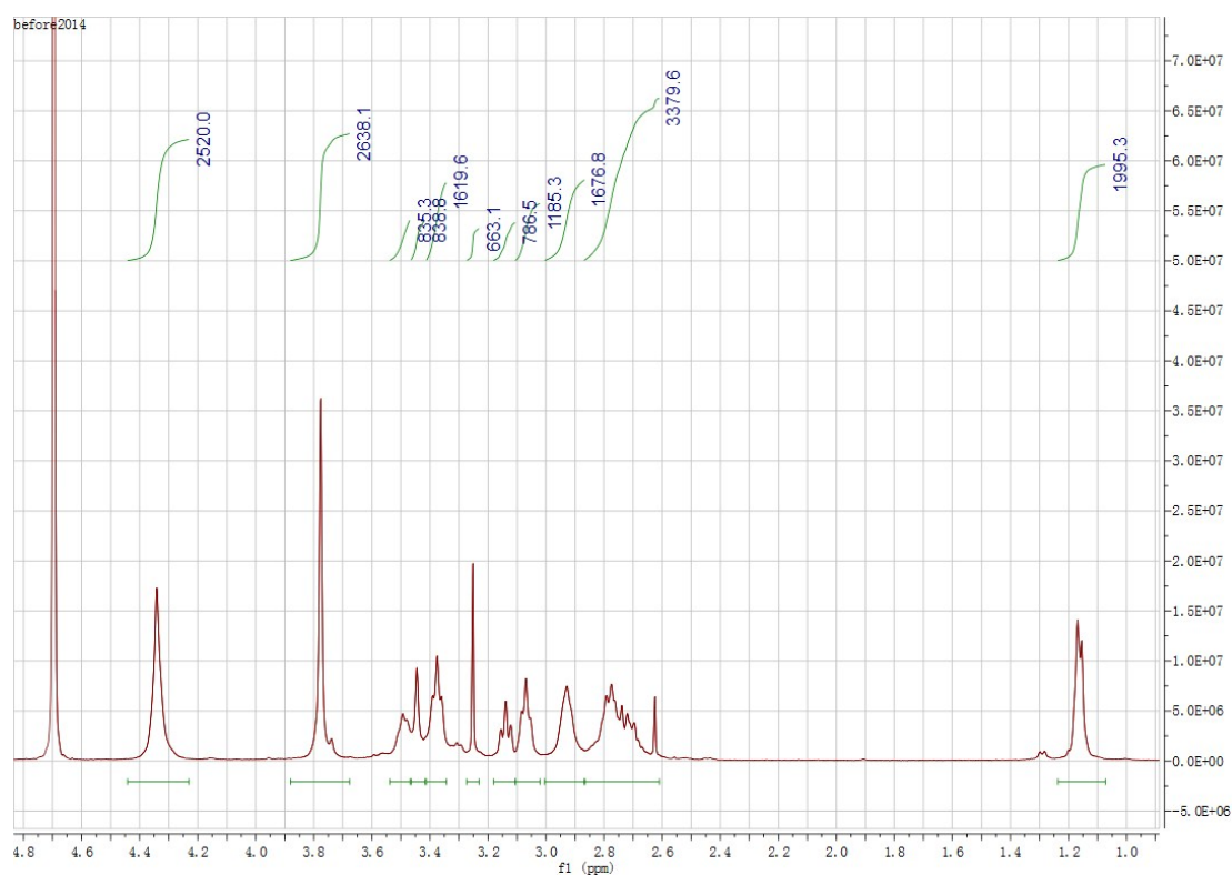
Figure S3. 1 H NMR spectrum of G4-DTPA in D 2 O.
