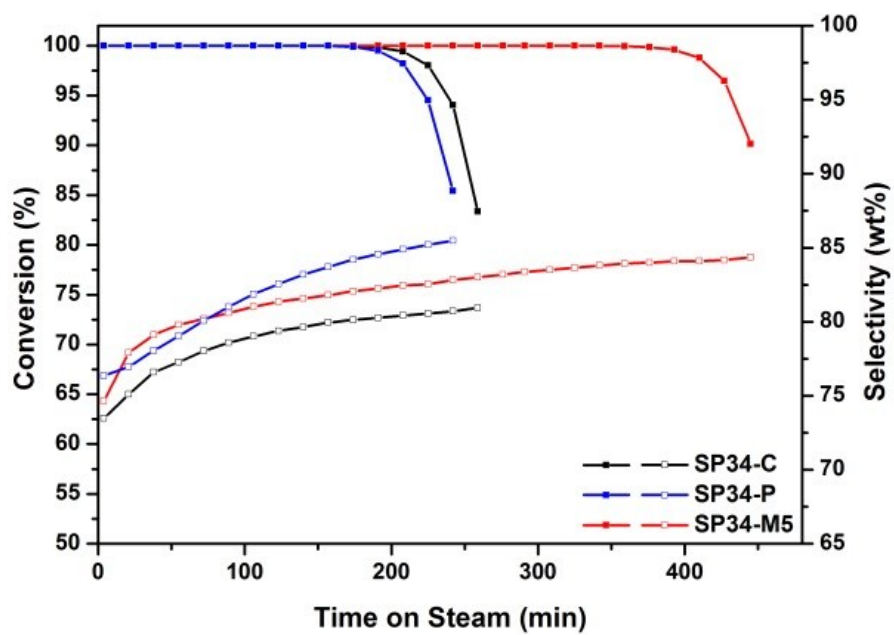
Fig. S4 Methanol conversion (solid) and ( C_2H_4+C_3H_6 ) selectivity (hollow) variation with time-on-stream over samples. Experimental conditions: WHSV = 2\text{ h}^{-1} , T = 450\text{ }^\circ\text{C} , catalyst weight= 300 mg.
