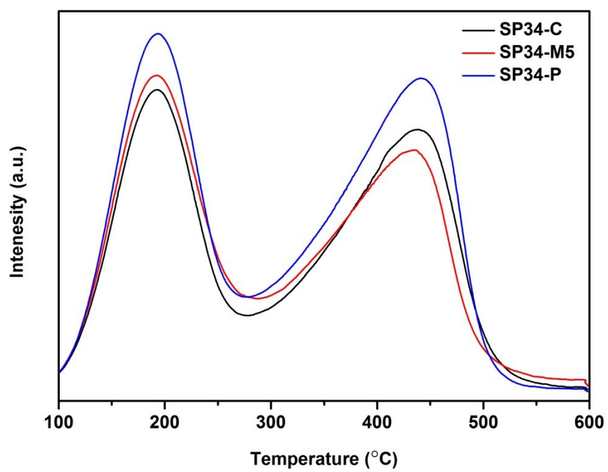
Fig. S5 NH 3 -TPD profiles of samples.
