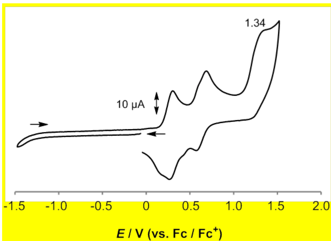
Figure S3. Cyclic voltammogram of 1^{\text{H}} (1.0 mM) in a \text{CH}_2\text{Cl}_2 solution containing 0.10 M n\text{Bu}_4\text{NPF}_6 (working electrode = GC, counter electrode = Pt, scan rate = 0.1 \text{ V s}^{-1} ).
