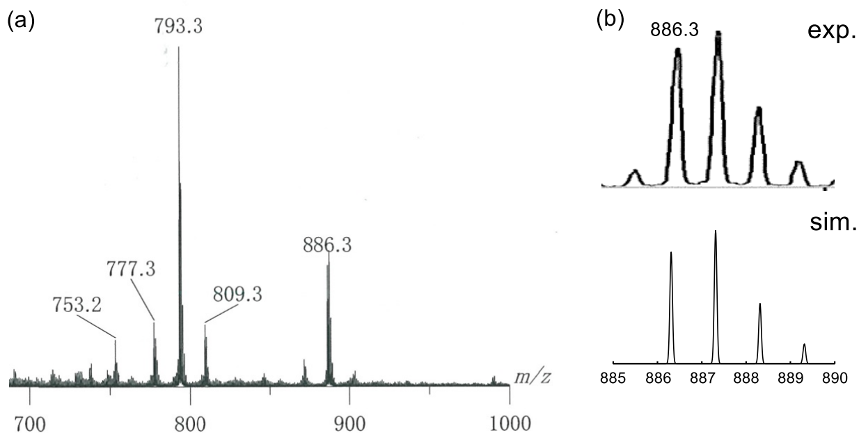
Figure S7. (a) FAB-MS (positive ion mode) spectrum of a reaction solution of 1 H with TsN 3 . (b) Enlarged view of the peaks at m/z = 887.3 . This isotope distribution patterns correspond to a 2:3 mixture of [\text{Rh}+\text{L}+\text{NTs}+\text{A}^{\text{H}}+\text{H}]^{+} and [\text{Rh}+\text{L}+\text{NTs}+\text{A}^{\text{H}}+2\text{H}]^{+} .
