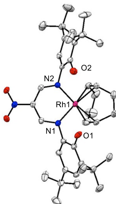
Figure S1. Crystal structure of \text{Rh}^{\text{I}}(\text{LH}_2^-)(\text{cod}) ( \text{cod} = 1,5\text{-cyclooctadiene} ). The solvent molecule (methanol) and hydrogen atoms are omitted for clarity.
