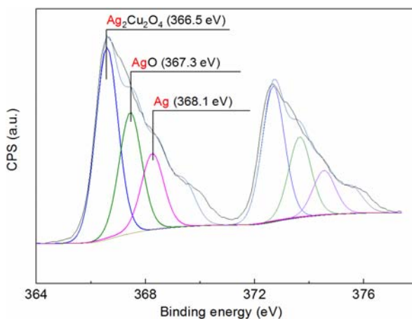
Supplementary Material 2: XPS deconvolution of the Ag 3 d 1/2 bands for Ag-Cu film 50%/50%
