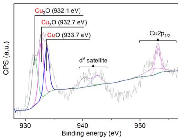
Supplementary Material 1: XPS deconvolution of the Cu 2 p 1/2 bands for the Ag-Cu film 50%/50%.
