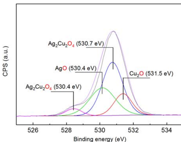
Supplementary Material 3: XPS O 1 s deconvolution in Ag-Cu film 50%-50%.
