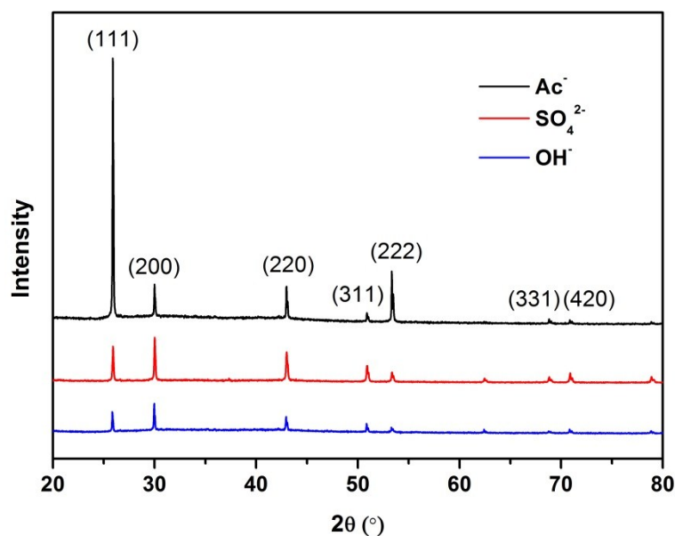
Figure S2 XRD patterns of the products prepared using different anions instead of Cl - .
