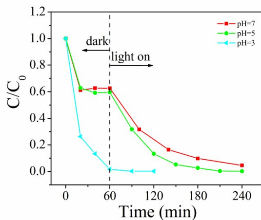
Figure S2. Degradation profiles of RhB solution under different pH values with sample S2 as photocatalyst. (a) pH=7; (b) pH=5; (c) pH=3.
