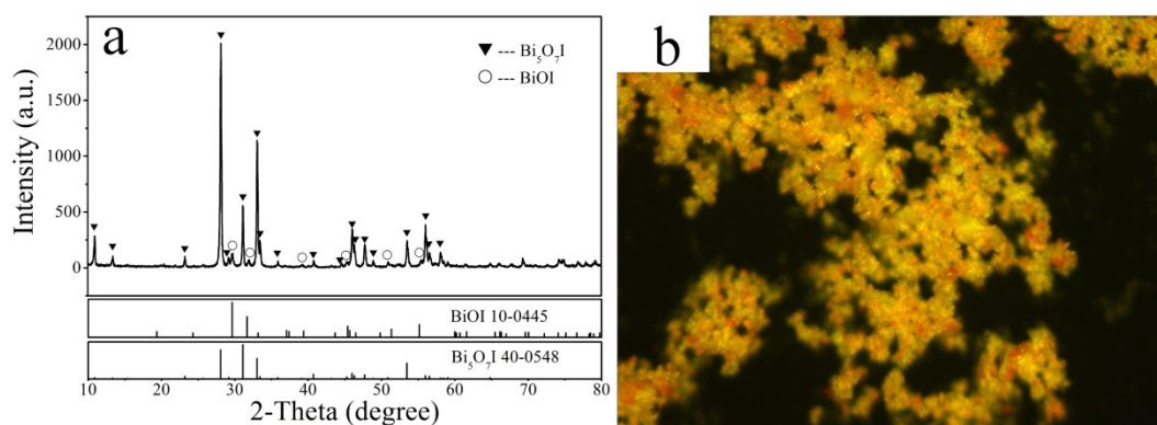
Figure S1. XRD pattern and optical microscope image of bismuth based sample with 1.9 g of NaOH introduction.
