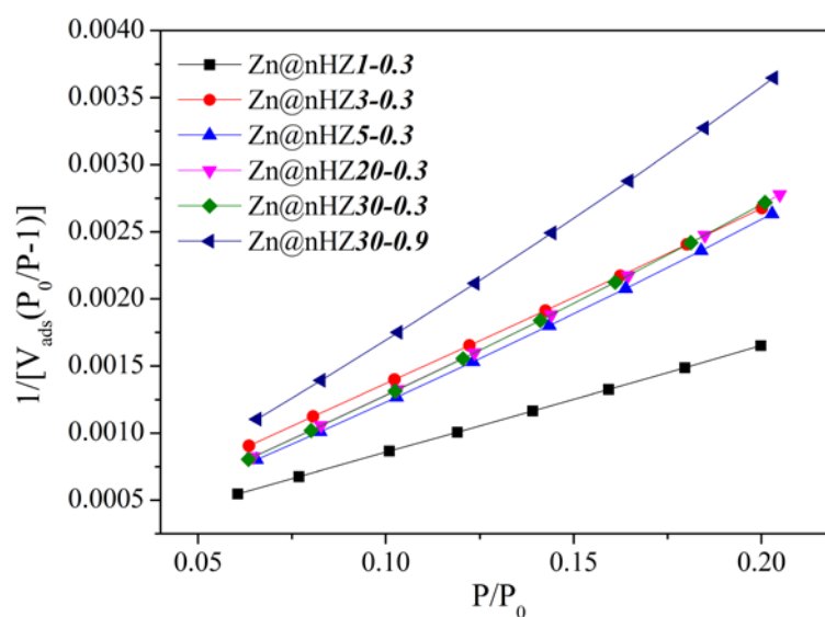
Fig.S1 BET plots of Zn@nHZx-y.
