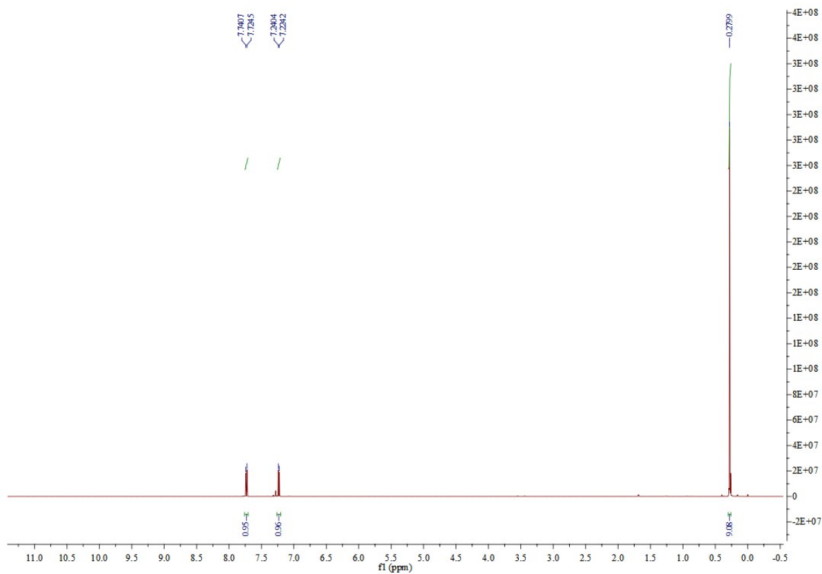
1 H NMR spectrum (CDCl 3 ) of compound 3 .
