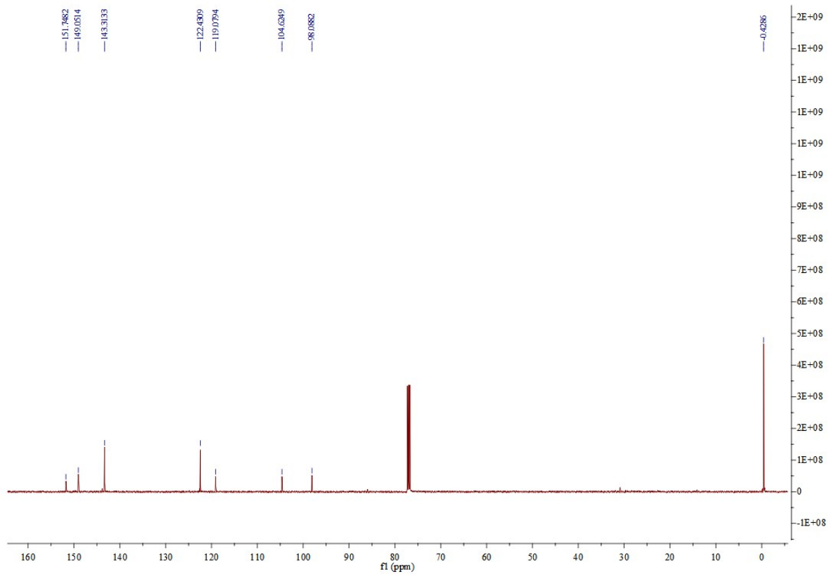
13 C NMR spectrum (CDCl 3 ) of compound 3 .
