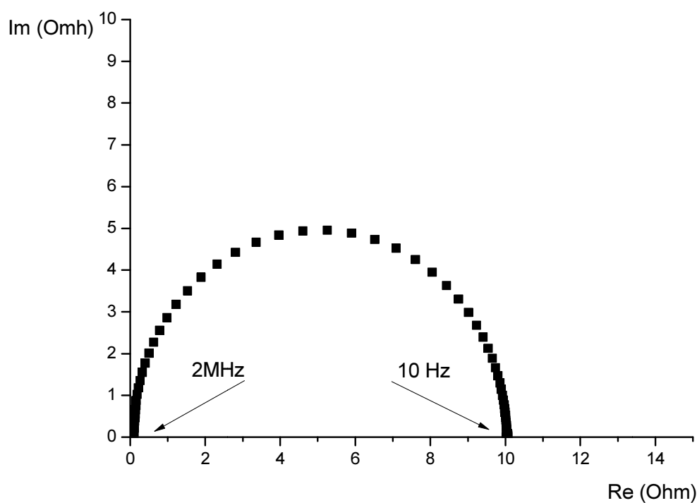
Figure 1s. The impedance spectrum of \text{Cp}_2\text{Fe}\dots\text{C}_2\text{I}_2 specimenes. Semi-circle shape of a curve signify the e-type conductivity.
