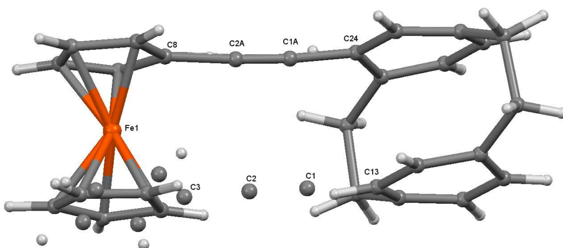
Figure 2s. Molecular structure of 1-paracyclophane-2-ferrocenylacetylene ( 6 ) showing disorder in the positions of Cp ring and triple C-C bond.
