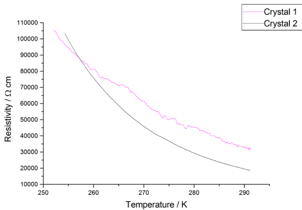
Fig. S4 Resistivity data for SS-1.Br
