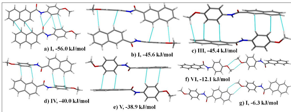
Figure S6: (a)-(g) Motifs I-VII present in the crystal packing of 6
