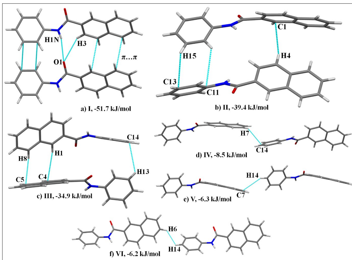
Figure S1: (a)-(f) Motifs I-VI present in the crystal packing of 1 .
