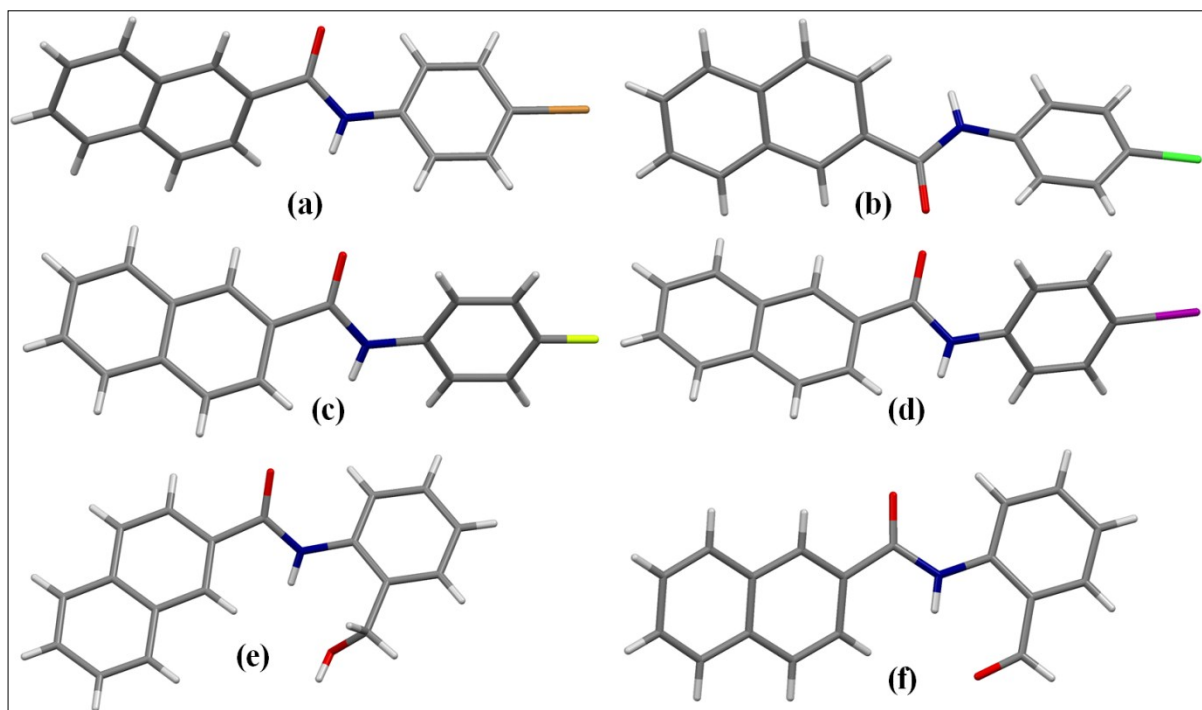
Figure S11: Structures of a) RIXGUC b) RIXHAJ c) RIXHEN d) RIXHIR e) XAFBOY and f) XAFCAL
