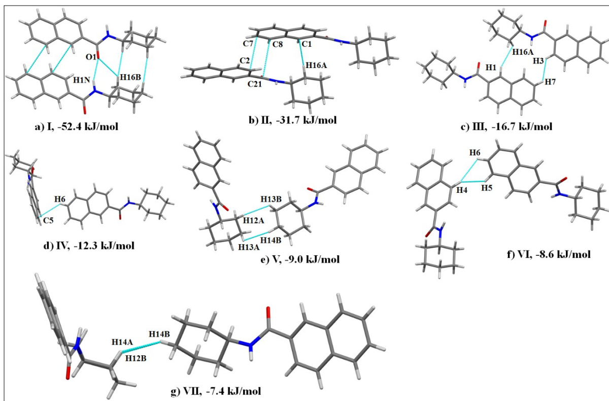
Figure S2: (a)-(g) Motifs I-VII present in the crystal packing of 2 .
