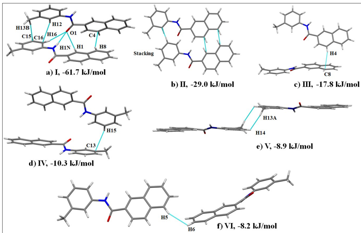
Figure S3: (a)-(f) Motifs I-VI present in the crystal packing of 3 .
