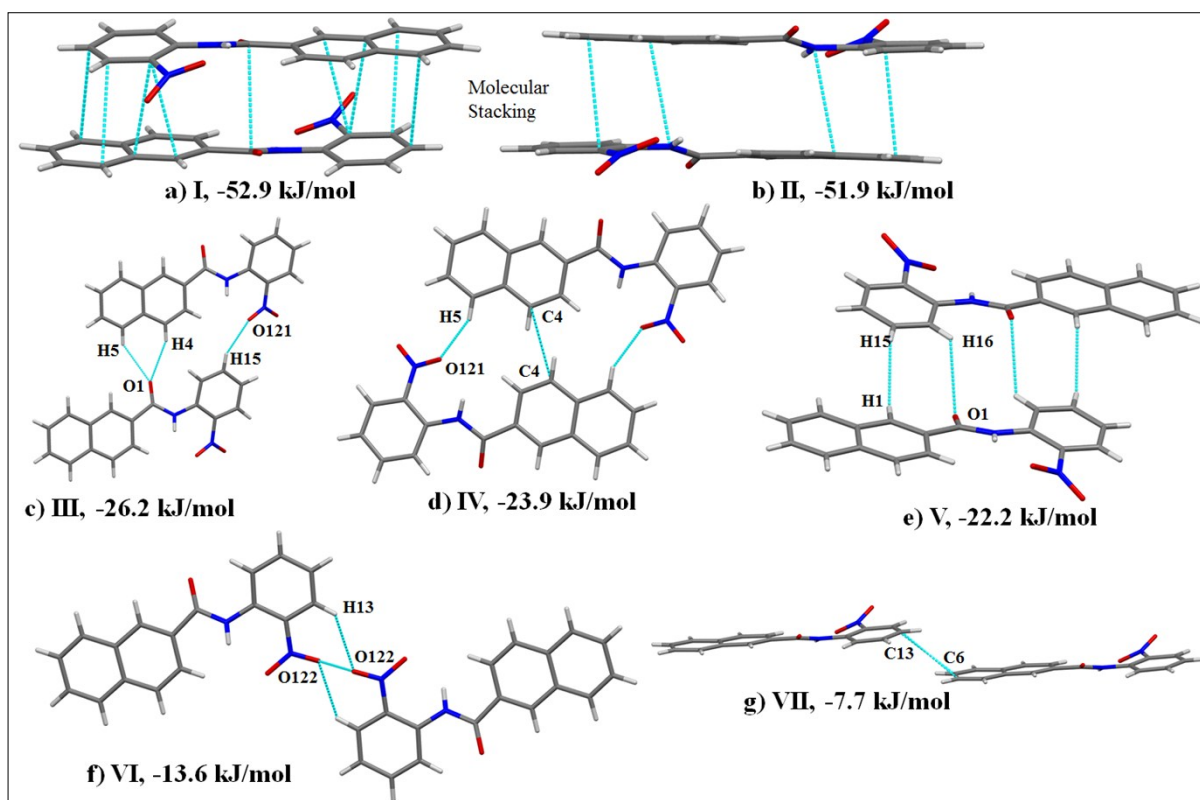
Figure S7: (a)-(g) Motifs I-VII present in the crystal packing of 7 .
