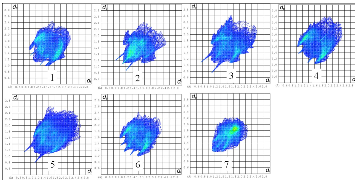
Figure S12: 2D Fingerprint plots for 1-7.
