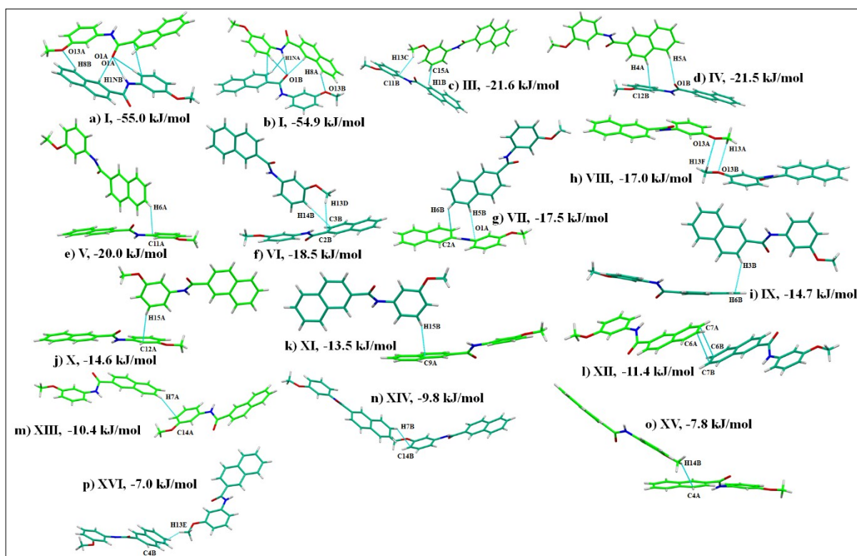
Figure S5: (a)-(p) Motifs I-XVI present in the crystal packing of 5 .
