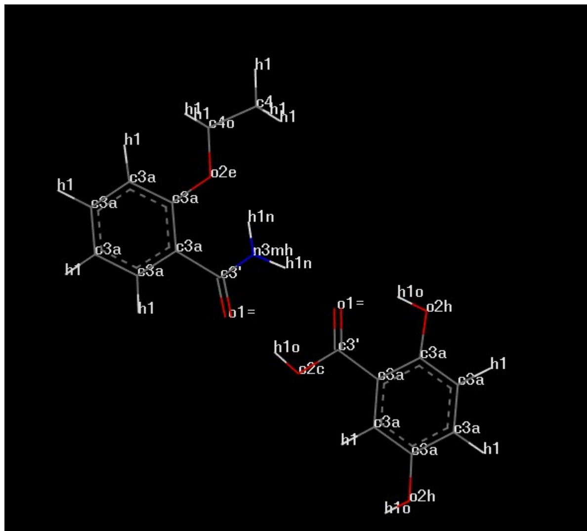
Fig. S6. QULLUF02 optimized asymmetric unit calculated using correct atom types.
