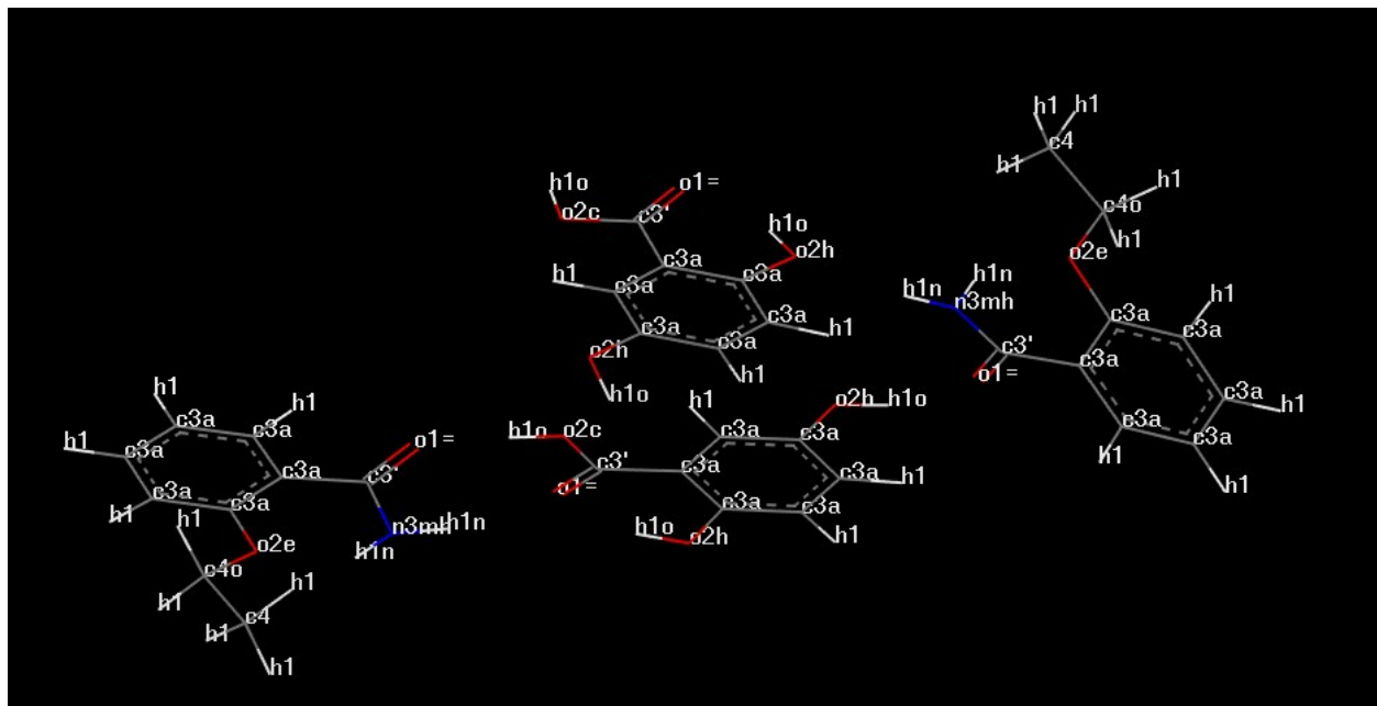
Fig. S2. QULLUF optimized asymmetric unit calculated using correct atom types.
