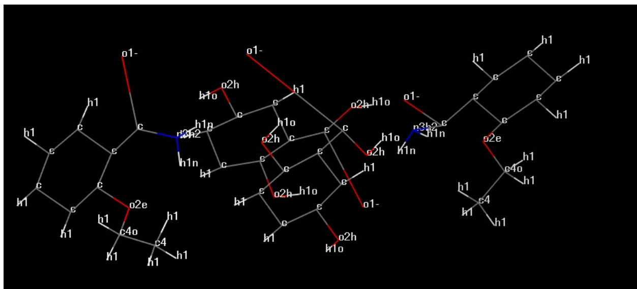
Fig. S1. QULLUF optimized asymmetric unit calculated using wrong atom types.
