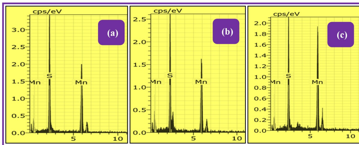
Fig. SI1: EDX spectra of \gamma -MnS films deposited at: (a) 60°C, (b) 80°C and (c) 100°C.
