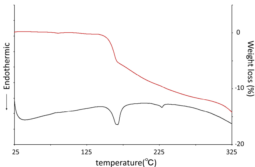
Fig. S1. TG (red) and DTA (black) curves of CH5134731 benzoic acid cocrystal.
