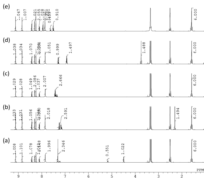
Fig. S2. 1 H-NMR (a)benzyl alcohol solvate, (b) toluene solvate, (c) chlorobenzene solvate, (d) anisole solvate, (e) benzoic acid cocrystal
