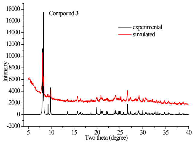
Fig. s3 simulated and experimental XRD patterns of compounds 1-3.
