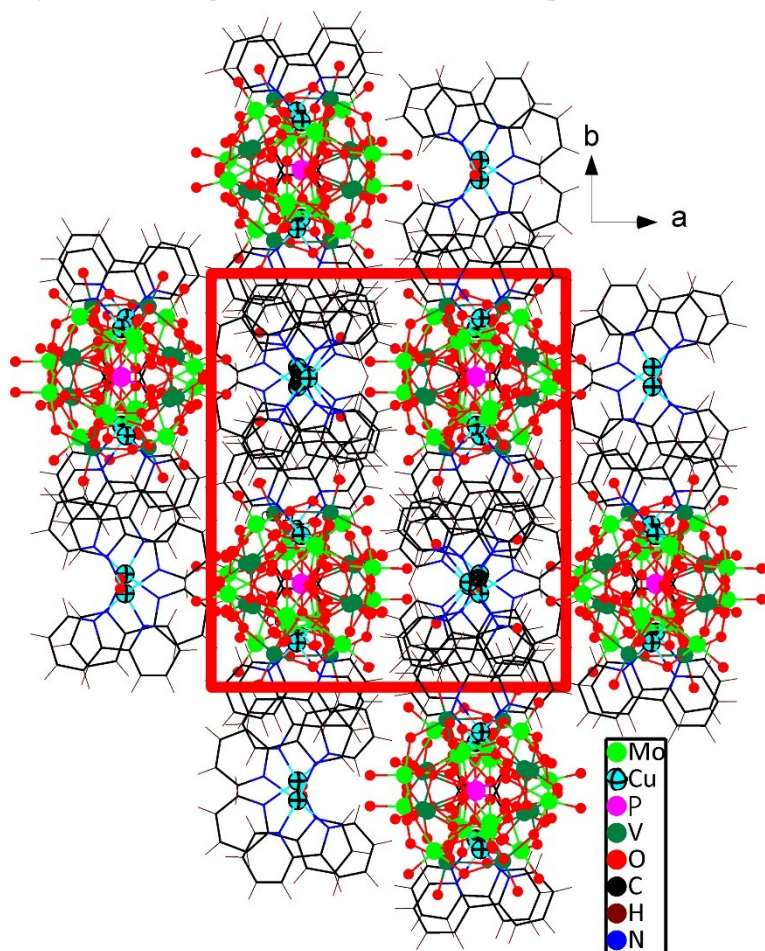
Fig. 2 the 3-D supramolecular structure of compound 2.
