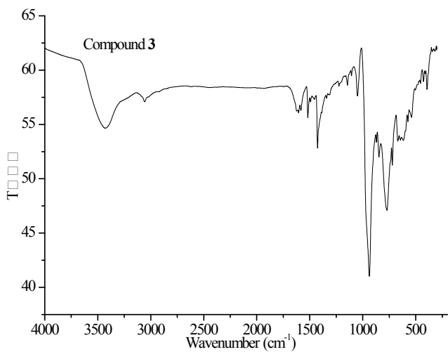
Fig. s4 IR spectra of compounds 1-3.
