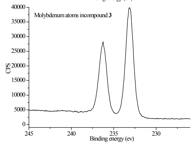
Fig. s7 XPS spectra of molybdenums in compounds 1-3.
