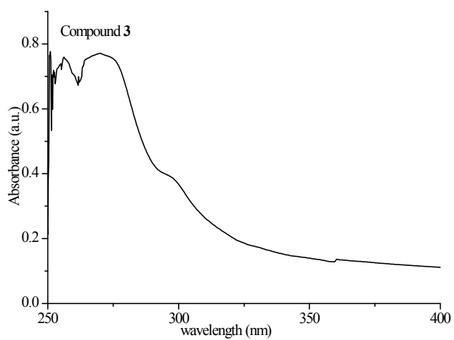
Fig. s5 UV-Vis spectra of compound 1-3.
