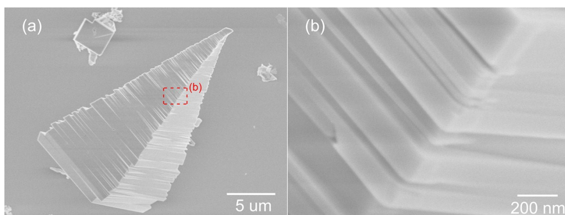
Fig.S1 (a) and (b) the low and high resolution SEM image of the SnSe pyramid structure.
