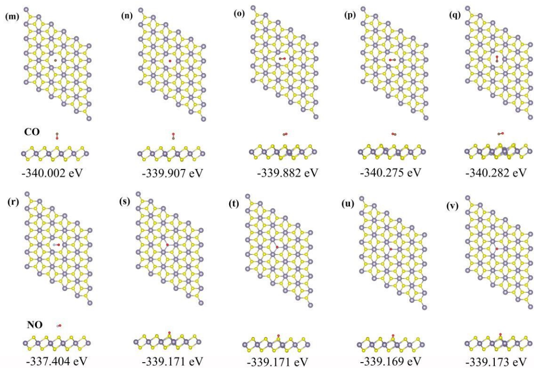
Figure S1. The models for gas molecule adsorbed s-vacancy SnS 2 monolayer systems in different configuration with corresponding adsorption energy.
