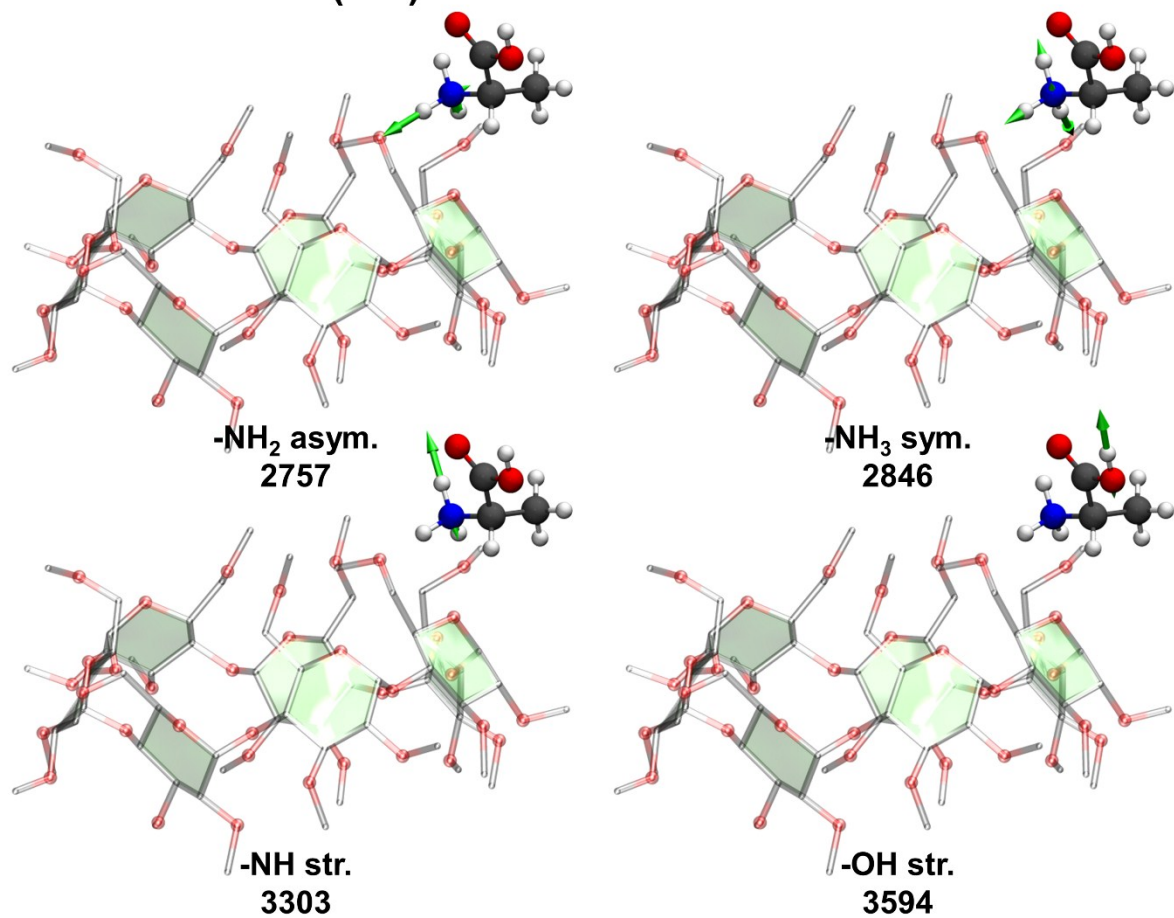
Figure 4S. Normal modes of the absorption bands of (L-2).
