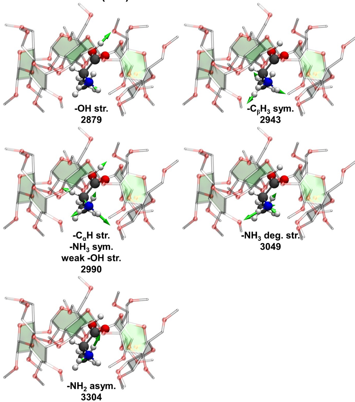
Figure 2S. Normal modes of the absorption bands of (D-3).
