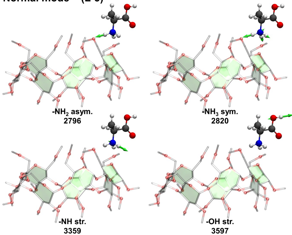
Figure 5S. Normal modes of the absorption bands of (L-3).
