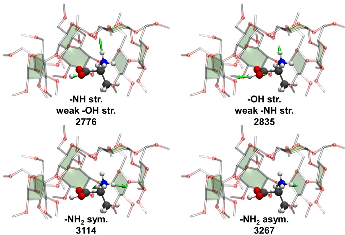
Figure 1S. Normal modes of the absorption bands of (D-2).
