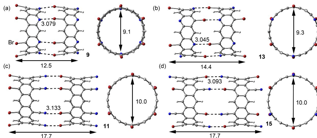
Fig. S1 (a-c) Optimized geometries of bromine dimeric complexes studied in this work. Distances in Å
