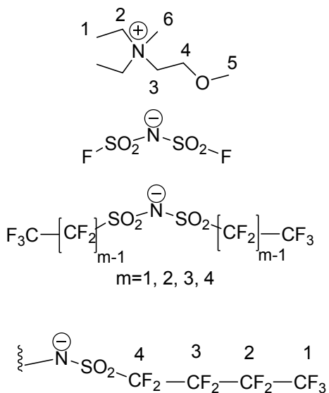
Scheme 1. Molecular structures and atom numbering for cation and anions of the ILs used in this work. From top to bottom: Sketch of DEME cation. Sketch of IM 00 anion. General formula for anions IM 11 -IM 44 . Atom numbering for the perfluoroalkyl chains, shown in the nonafluorobutyl case (m=4).
