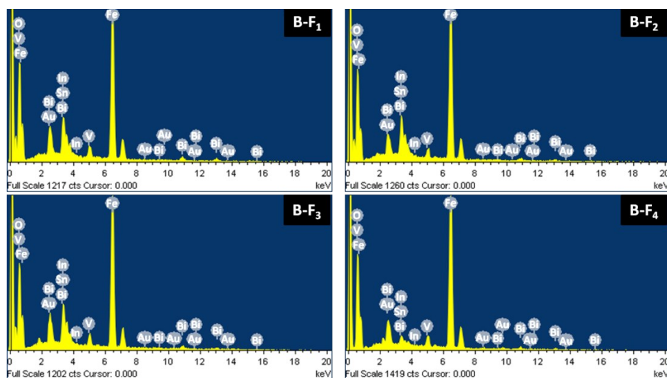
Fig. S1. EDX maps of heterojunction samples viz. B-F 1 , B-F 2 , B-F 3 and B-F 4
