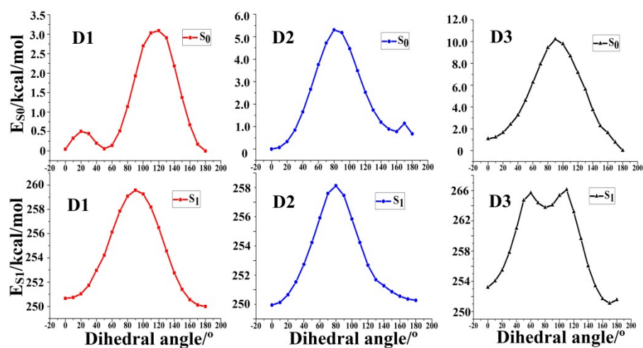
Figure 1: Potential energies curves of S 0 and S 1 states of n-butanol-NIAD-4 with three dihedral angles increase.
