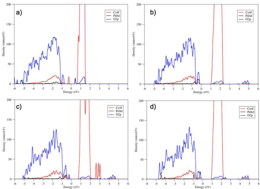
Figure S8. Density of states (DOS) plots of \text{Pd}_1\text{Ce}_{39}\text{O}_{79} . Plot a) corresponds to Pd located in D1 position, b) to D2, c) to D3 and d) to D4, respectively.
