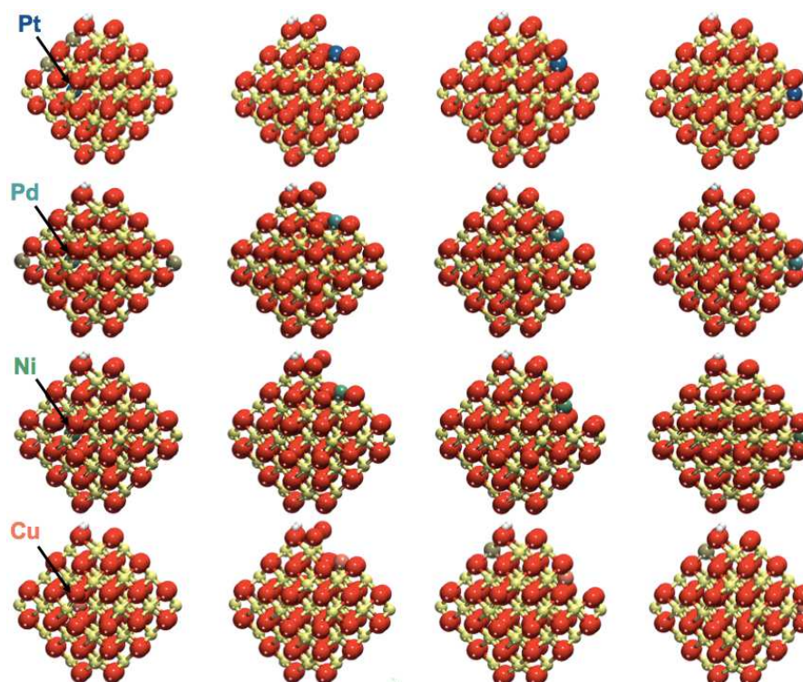
Figure S11. Overview of the most stable structures \text{H}_2\text{M}_1\text{Ce}_{39}\text{O}_{80} of systems formed upon dissociative adsorption of two hydrogen atoms in two nearby oxygen atoms of one of the \{100\} nanofacets.
