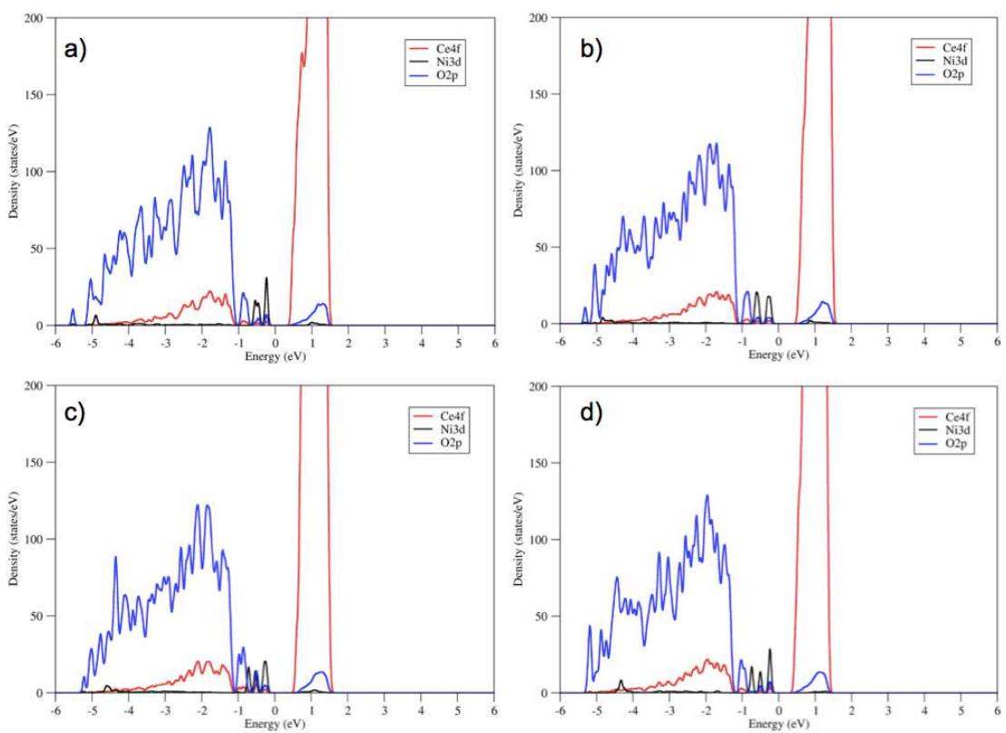
Figure S9. Density of states (DOS) plots of \text{Ni}_1\text{Ce}_{39}\text{O}_{79} . Plot a) corresponds to Ni located in D1 position, b) to D2, c) to D3 and d) to D4, respectively.
