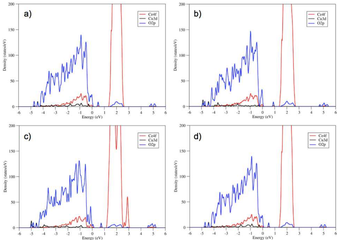
Figure S5. Density of states (DOS) plots of stoichiometric \text{Cu}_1\text{Ce}_{39}\text{O}_{80} . Plot a) corresponds to Cu located in D1 position, b) to D2, c) to D3 and d) to D4, respectively.
