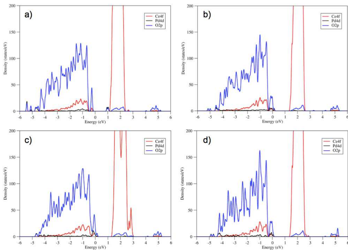
Figure S3. Density of states (DOS) plots of stoichiometric \text{Pd}_1\text{Ce}_{39}\text{O}_{80} . Plot a) corresponds to Pd located in D1 position, b) to D2, c) to D3 and d) to D4, respectively.
