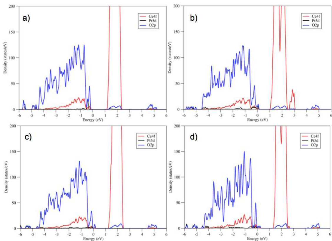
Figure S2. Density of states (DOS) plots of stoichiometric \text{Pt}_1\text{Ce}_{39}\text{O}_{80} . Plot a) corresponds to Pt located in D1 position, b) to D2, c) to D3 and d) to D4, respectively.
