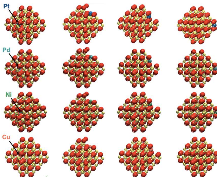
Figure S1. Stoichiometric M_1Ce_{39}O_{80} structures formed by the substitution of a Ce^{4+} cation by a transition metal (M) atom. The M atoms are located in four different positions (D1, D2, D3 and D4) of the ceria nanoparticle.
