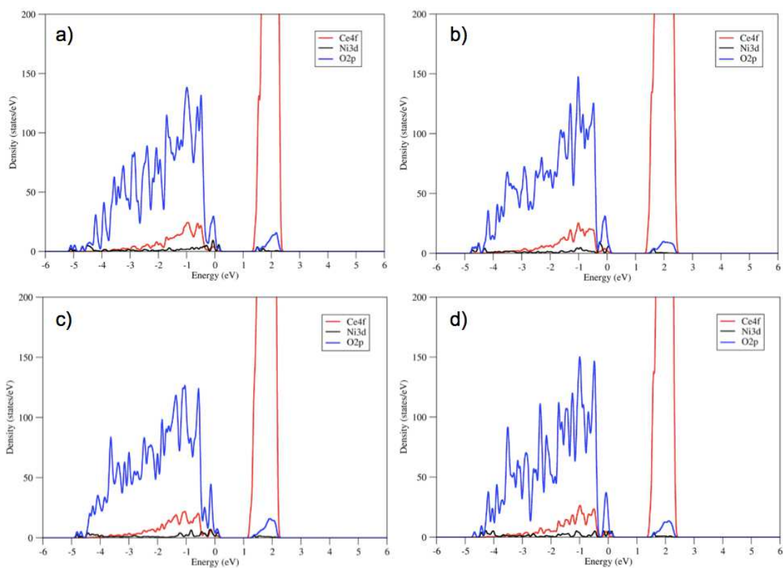
Figure S4. Density of states (DOS) plots of stoichiometric \text{Ni}_1\text{Ce}_{39}\text{O}_{80} . Plot a) corresponds to Ni located in D1 position, b) to D2, c) to D3 and d) to D4, respectively.
