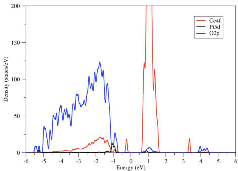
Figure S7. Density of states (DOS) plot of Pt_1Ce_{39}O_{79} corresponding to Pt located in D1 position.
