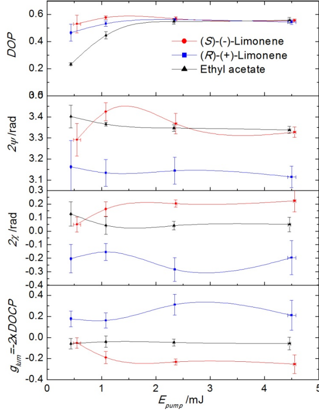
Figure S3: Laser emission polarization state parameters as a function of pump energy for a linear 45° pump polarization. Each point and error bar represents the average and standard deviation, respectively, of the fitting parameters obtained over 4 sets of measurements. Lines are guides to the eye.
