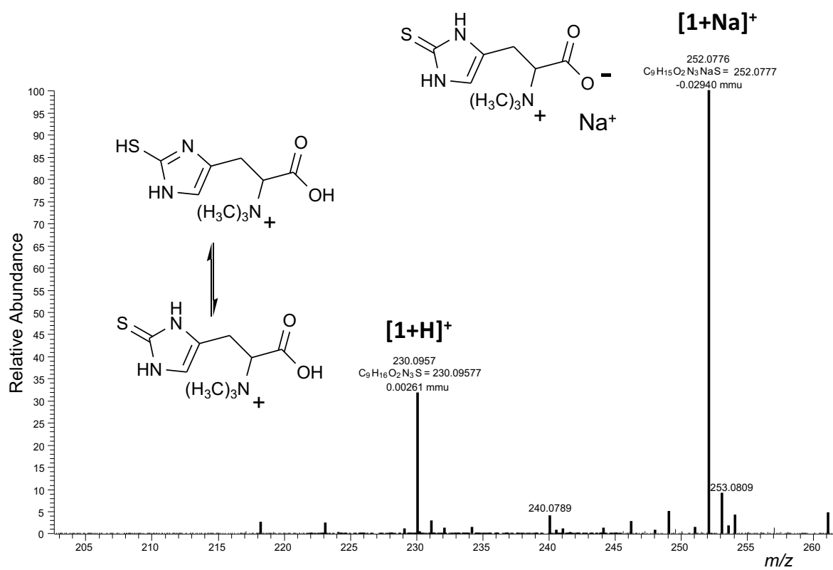
Figure S1. (+)ESI-MS of Ergothioneine, MeOH
