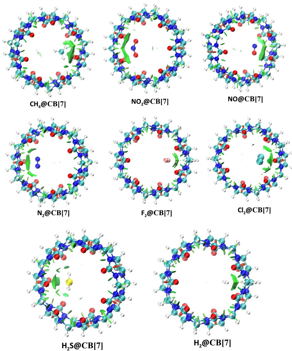
Fig. 1-SI NCI isosurface plots of gas@CB[7] at the \omega B97X-D/6-311+G(d,p) level.
