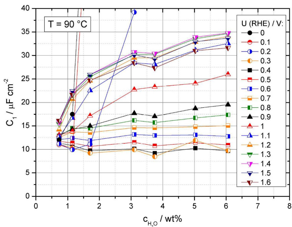
Fig. S1: C_1 vs. water content, influence of potential, data taken from Fig. 4.
