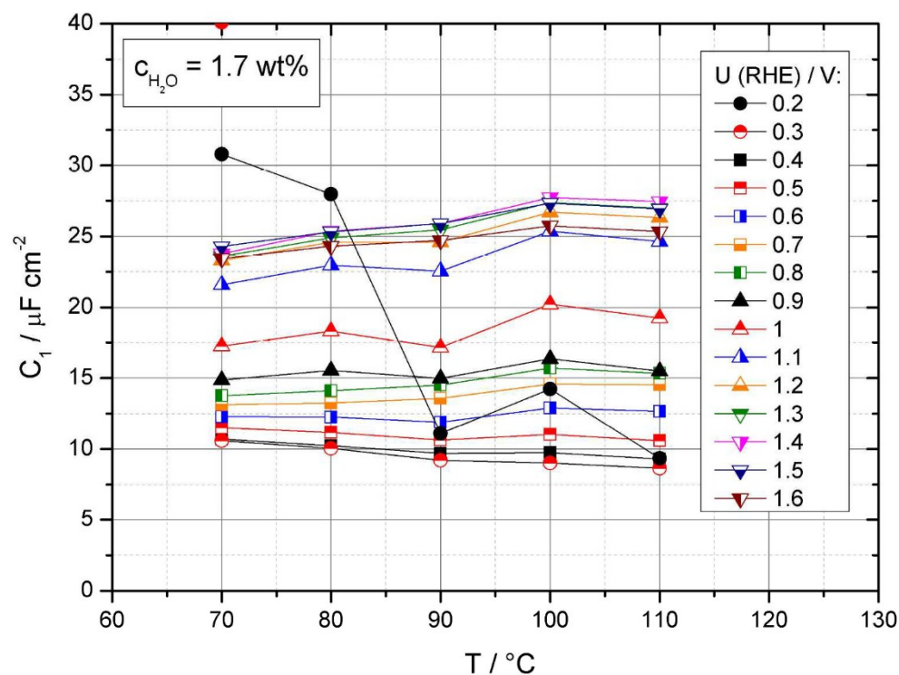
Fig. S2: C_1 vs. temperature, influence of potential, data taken from Fig. 5.
