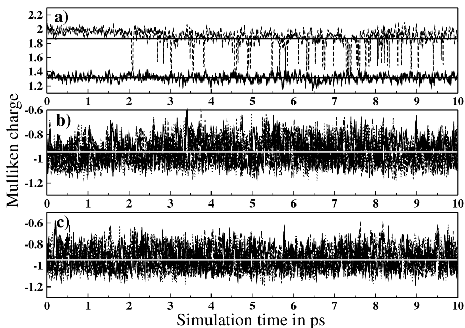
Figure S1: Fluctuation of partial atomic charges of a) \text{Fe}^{2+} (bold) and \text{Fe}^{3+} (dashed) and nitrogen partial charges of b) ferrous and c) ferric porphyrin obtained via QMCF-MD simulations+. Horizontal lines represent the respective average values.
