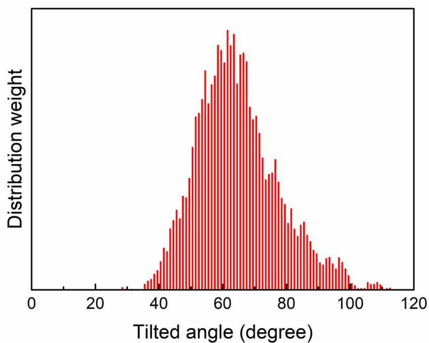
Fig. S1. The calculated tilted angle dependence of weight distribution of CO on the CO-CO 2 co-adsorbed a-TiO 2 (101) surface.
