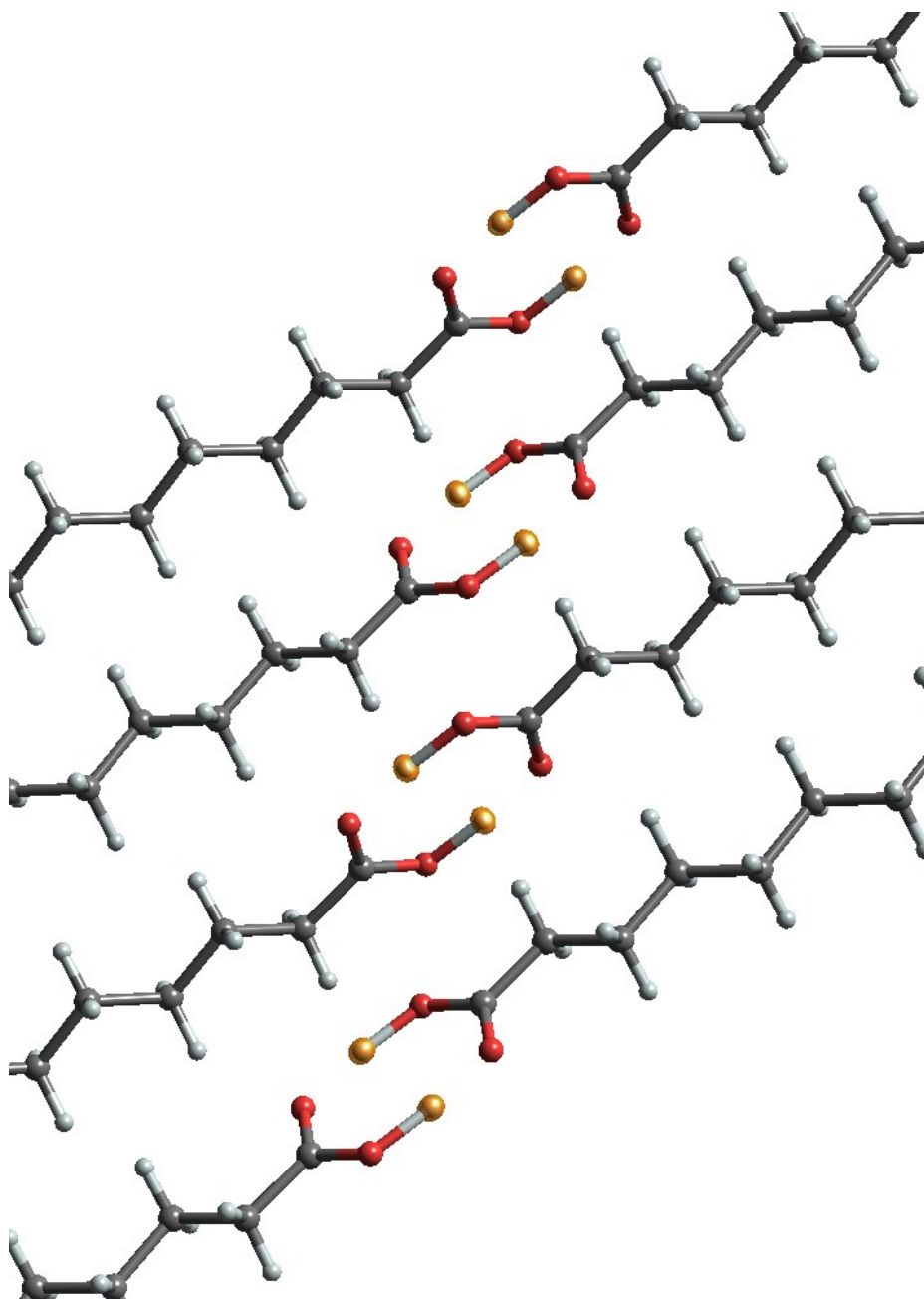
Figure 1. A TensorView illustration of palmitic acid phase C showing COOH hydrogen anisotropic displacement ellipsoids.
