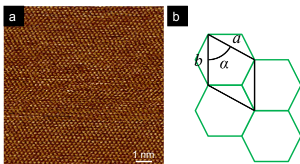
Figure S1. (a) Observed STM image of HOPG at a scanning condition ( I_{\text{set}} = 600 pA, V_{\text{bias}} = 10 mV). (b) Illustration of the graphite lattice.
