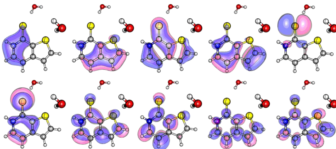
Fig. S1: Molecular orbitals used for the active space of CASSCF and MS-CASPT2 calculations.
