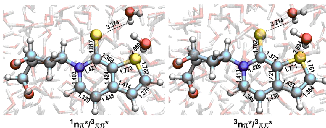
Fig. S2: Optimized structures of minimum-energy crossing point and conical intersection. Also shown are selected bond lengths (in Å) optimized at the QM(CASSCF)/MM level.
