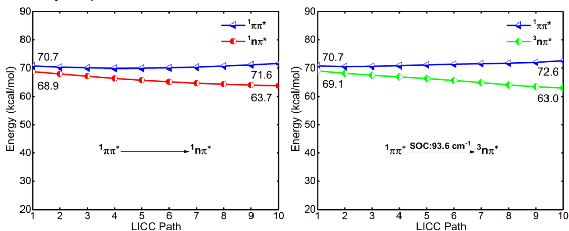
Fig. S3: QM(MS-CASPT2)/MM computed linearly interpolated Cartesian coordinate paths (LICCs, in kcal/mol) connecting (left) the S_2(1\pi\pi^*) and S_1(1n\pi^*) minima and (right) the S_2(1\pi\pi^*) and T_2(3n\pi^*) minima.
