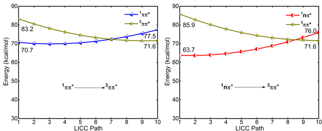
Fig. S4: QM(MS-CASPT2)/MM computed linearly interpolated Cartesian coordinate paths (LICCs, in kcal/mol) connecting (left) the S_2(1\pi\pi^*) and T_3(3\pi\pi^*) minimum and (right) the S_1(1n\pi^*) and T_3(3\pi\pi^*) minima.
