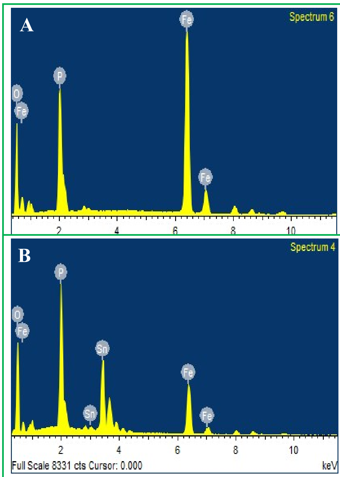
Figure S1: EDS results of FeHP and Sn-FeHP prepared by hydrothermal method
