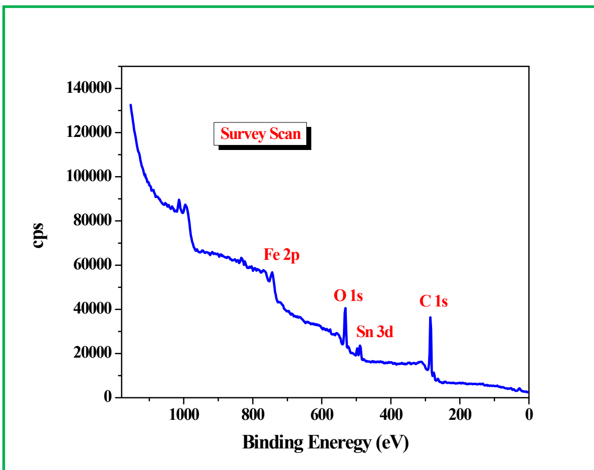
Figure S2: The survey scan of Sn-FeHP obtained from X-ray photoelectron spectroscopic analysis.
