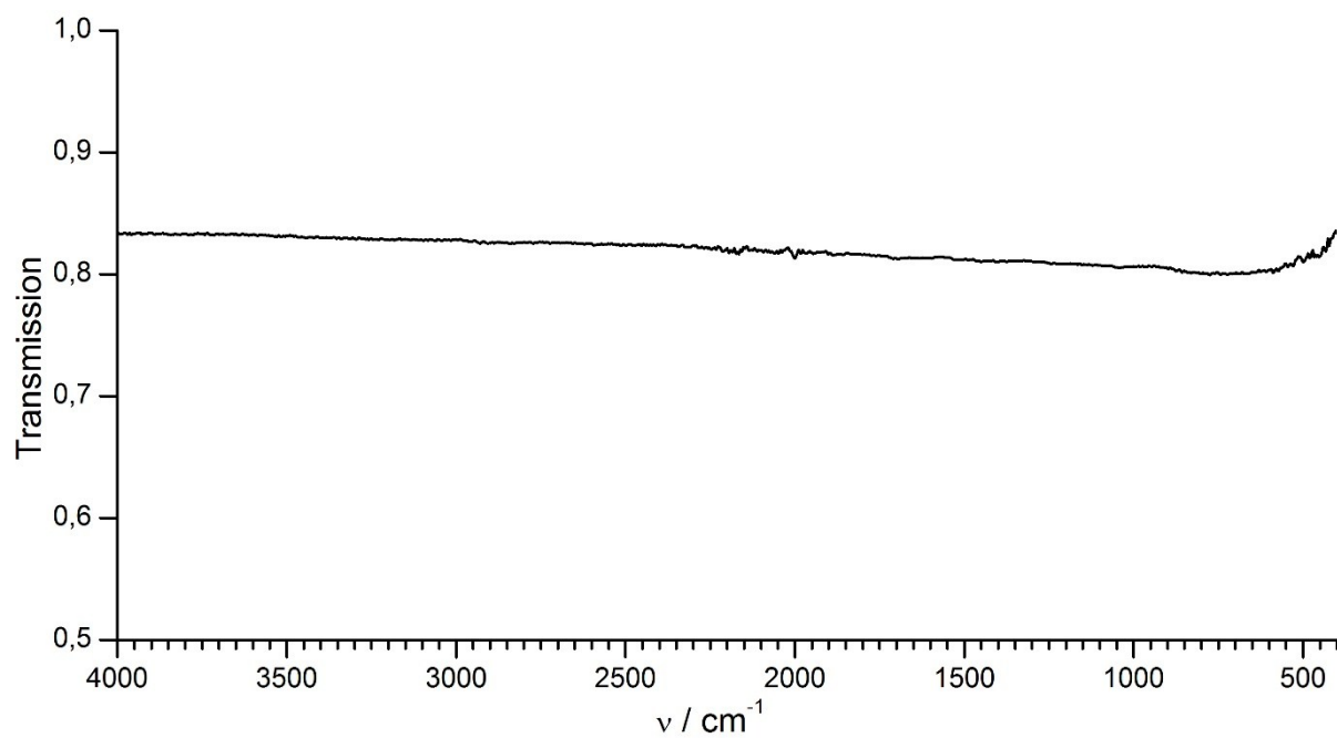
Figure S1. Diamond ATR-FTIR spectrum of \text{UCl}_4 .
