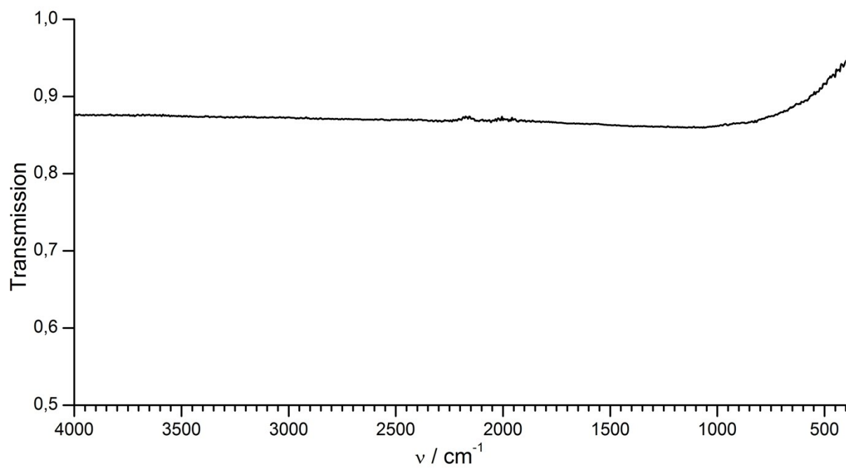
Figure S2. Diamond ATR-FTIR spectrum of \text{UBr}_4 .
