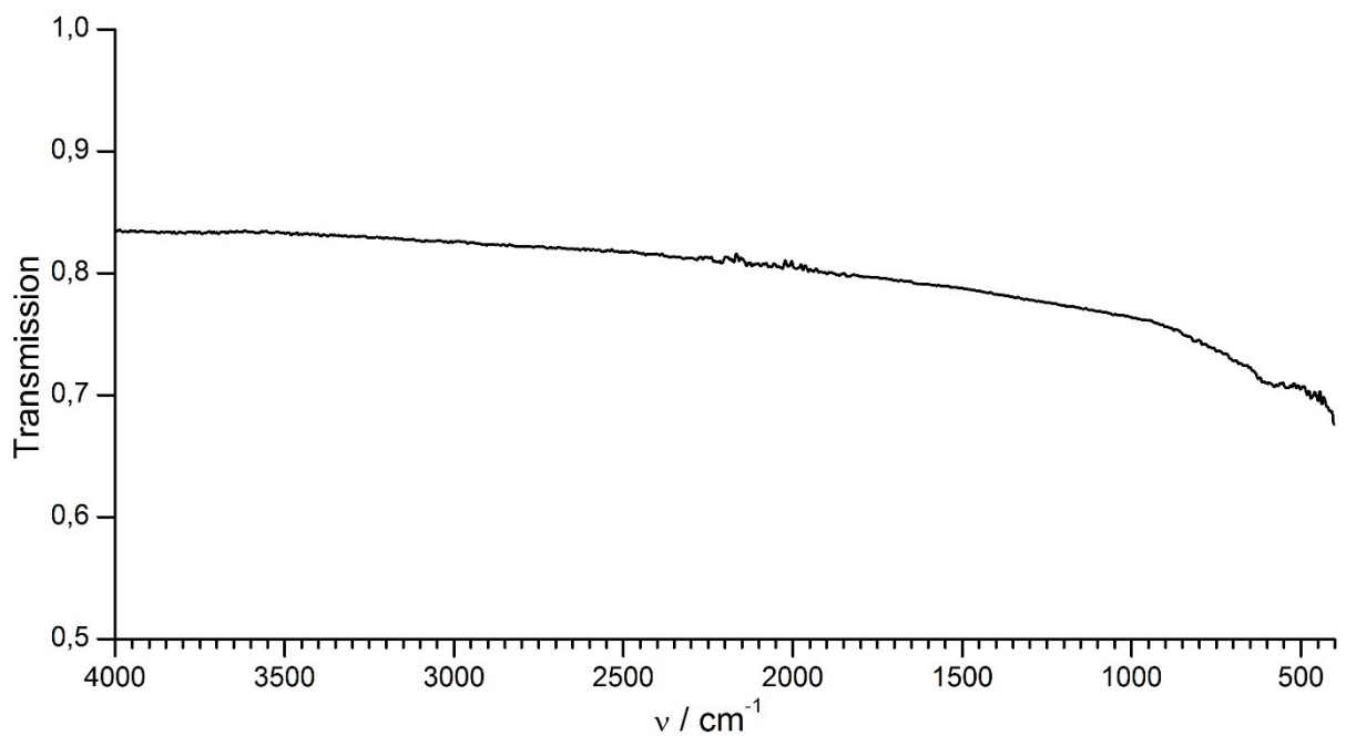
Figure S3. Diamond ATR-FTIR spectrum of UI 4 .
