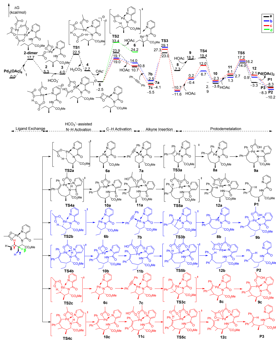
Fig. S1 Complete free energy profiles for the Pd(II)-catalyzed C(sp 3 )-H alkenylation of aliphatic amines. Energies are relative to Pd 3 (OAc) 6 + 1 + 2a and are mass balanced
