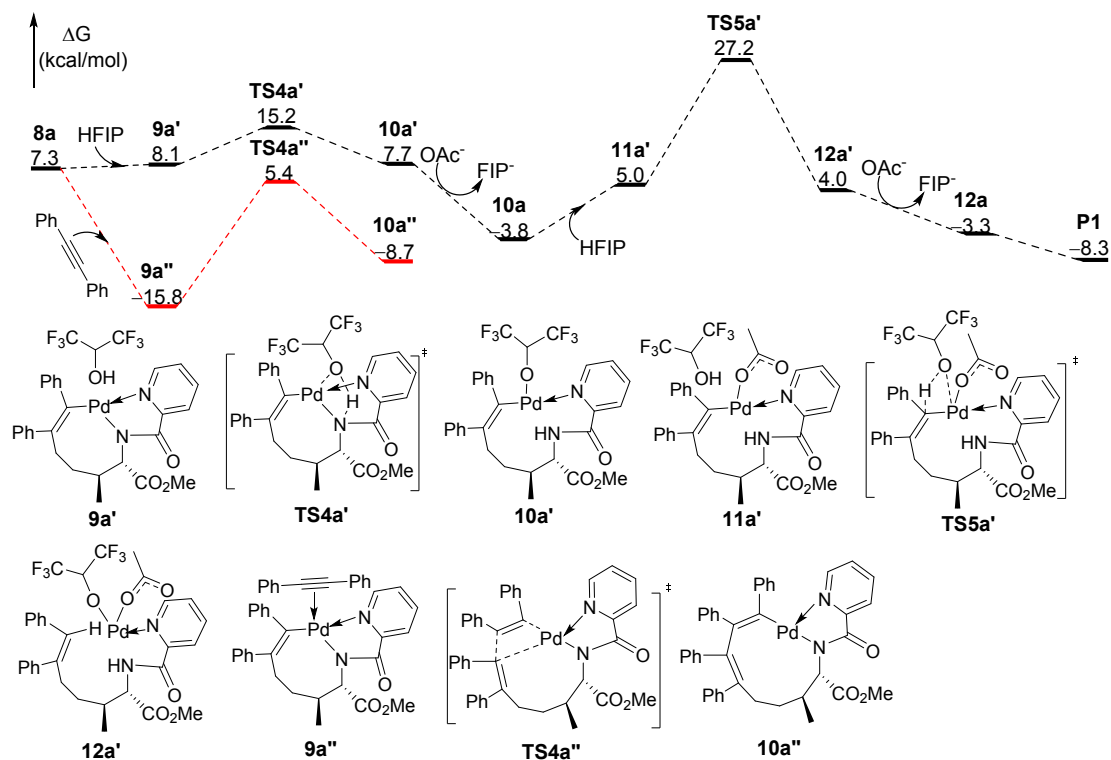
Fig. S5 Free energy profiles for the second insertion at 8a and two consecutive protonation steps to afford P1 using HFIP as the proton source. Energies are relative to Pd 3 (OAc) 6 +1+2a and are mass balanced.
