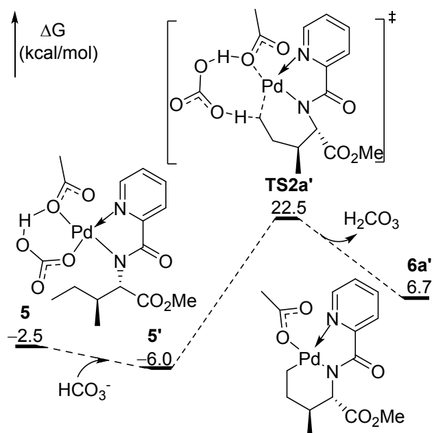
Fig. S3 Free energy profiles for the \text{HCO}_3^- -assisted C–H activation at the \delta -site. Energies are relative to \text{Pd}_3(\text{OAc})_6 + \mathbf{1} + \mathbf{2a} and are mass balanced.
