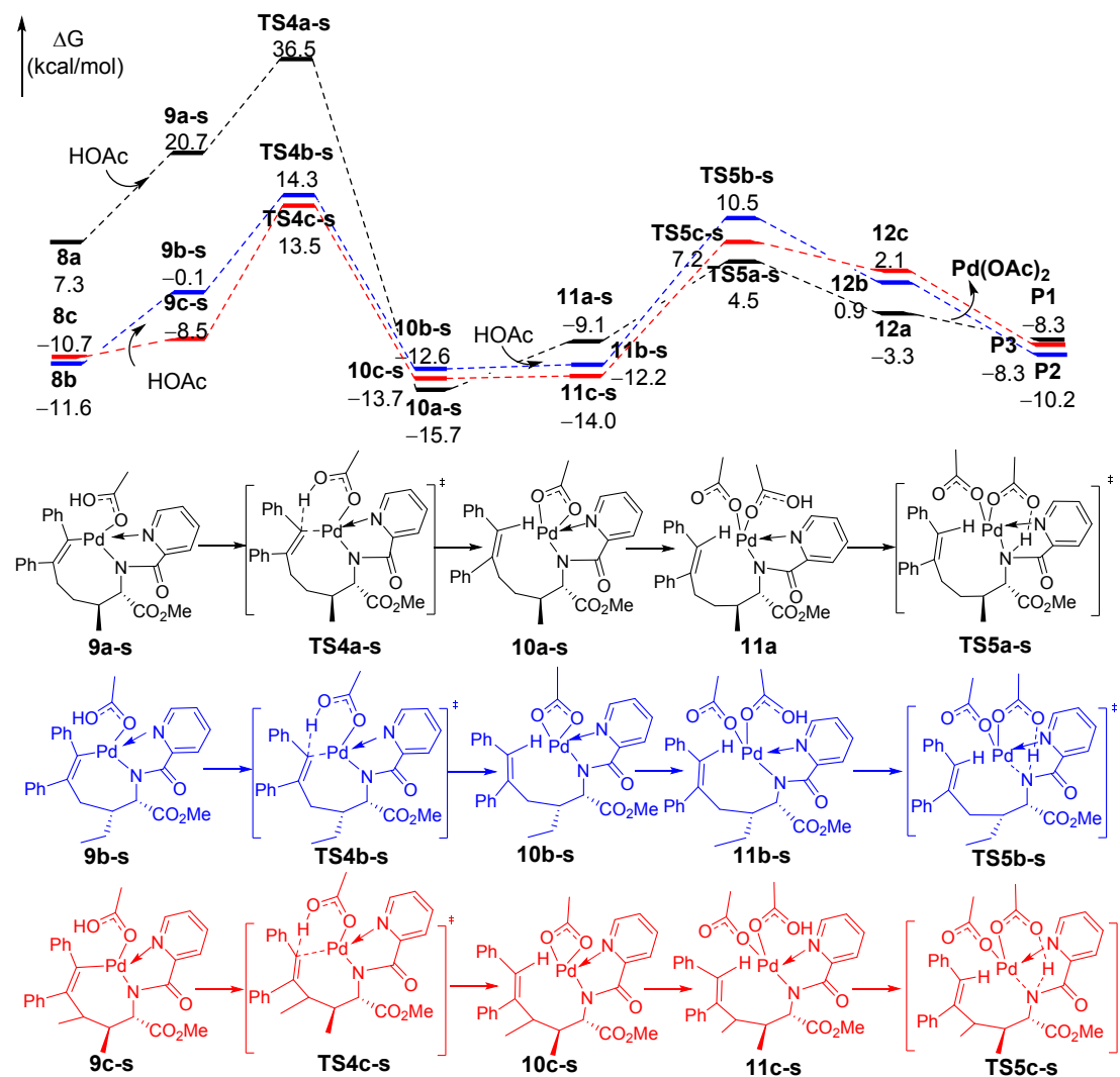
Fig. S4 Free energy profiles for another parallel pathway of the two consecutive protonation steps to afford the final products. Energies are relative to \text{Pd}_3(\text{OAc})_6 + \mathbf{1} + \mathbf{2a} and are mass balanced.
