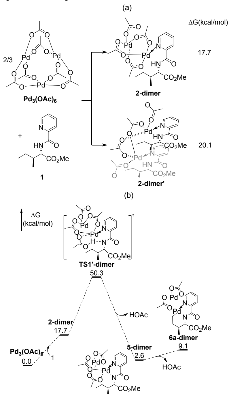
Fig. S2 (a) Two possible dimeric palladium complexes; (b) Free energy profiles for N-H activation of 2-dimer .
