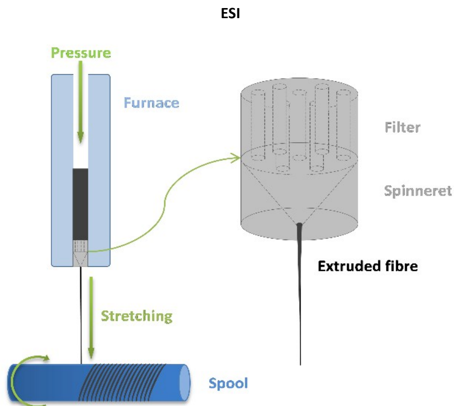
Figure 1SI. Melt-spinning principle used to produce green fibers.
