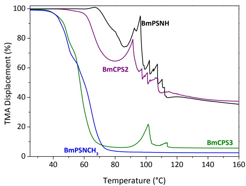
Figure 3SI. TMA curves for BmCPS1→3 , BmPSNCH 3 .
