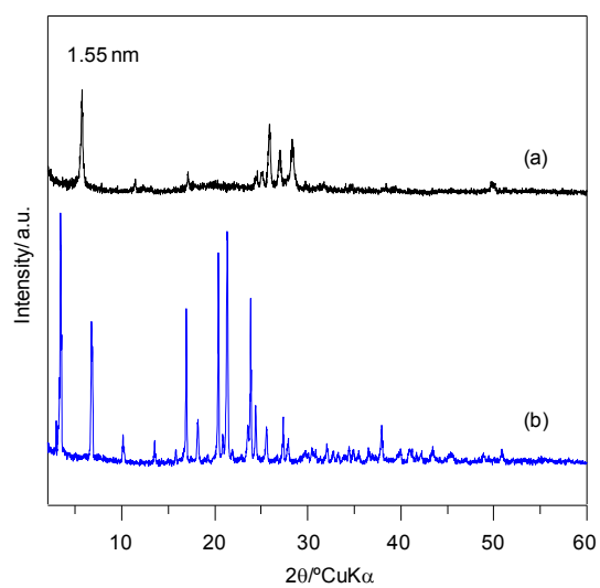
Figure S1. XRD patterns of magadiite (a), CTA (b).
