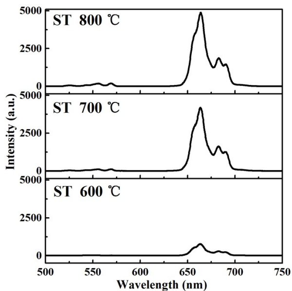
Fig. S1 UCL spectra of ST- \text{Sc}_2\text{O}_3: 10\% \text{Yb}^{3+}, 1\% \text{Er}^{3+} samples at different annealed temperatures (600, 700, and 800 °C).
