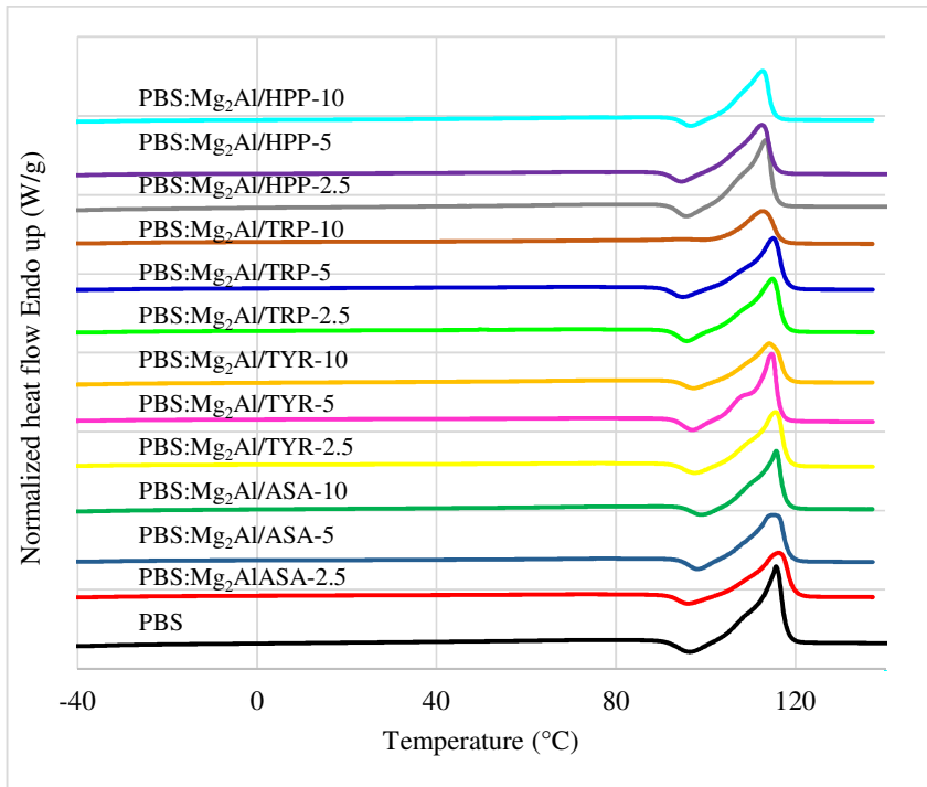
FIGURE S2. DSC traces of in situ PBS nanocomposites (heating scans and cooling scans)
