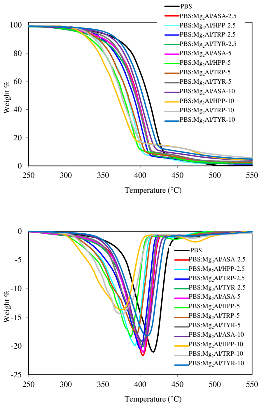
FIGURE S1. TGA and DTGA traces of in situ PBS nanocomposites
