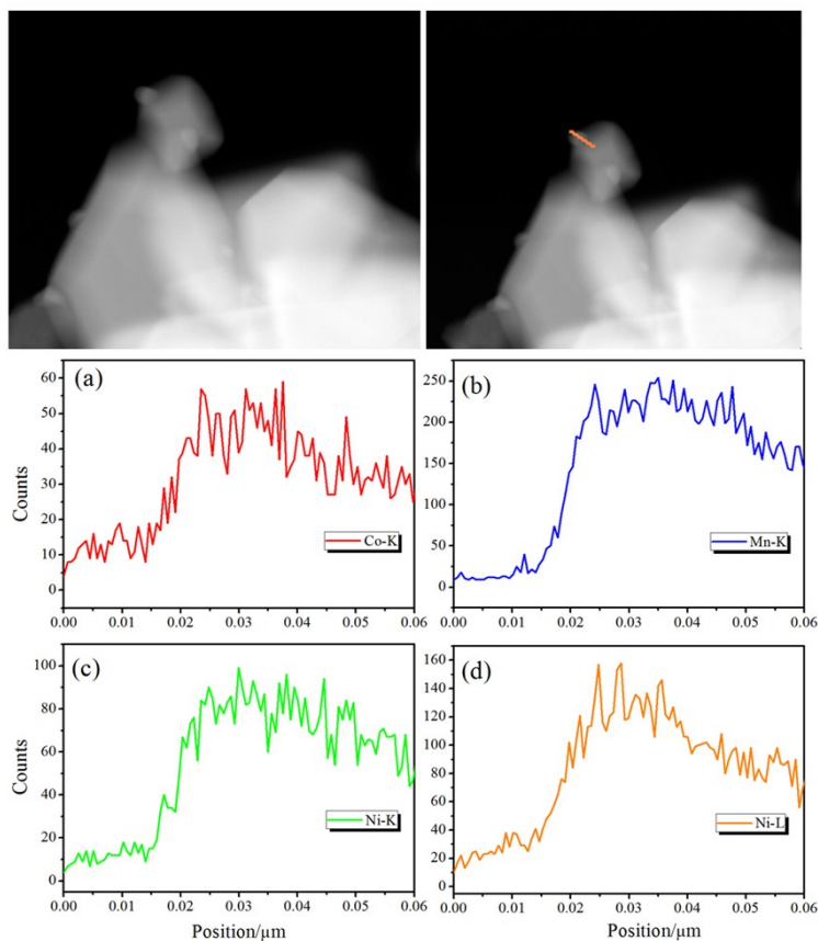
Fig. S2 The elemental distribution of LNMO@LC-10% obtained from EDS line-scan analysis.
