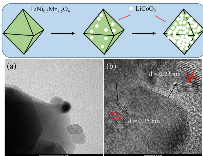
Fig. S1 The TEM and HRTEM images of LNMO@LC-10% sample.
