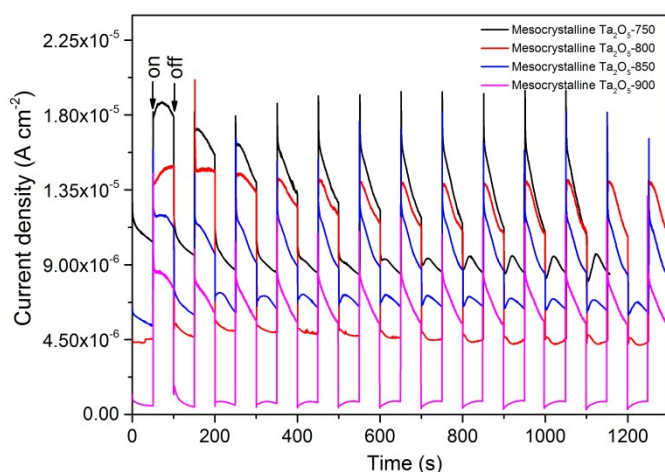
Fig. S1 Transient photocurrent response of mesocrystalline Ta 2 O 5 nanosheets.
