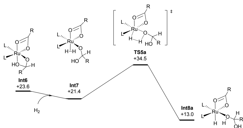
Figure S6. Energy profiles of the alternative H 2 heterolysis of Int6 . Gibbs free energies (kcal/mol) are relative to II .
