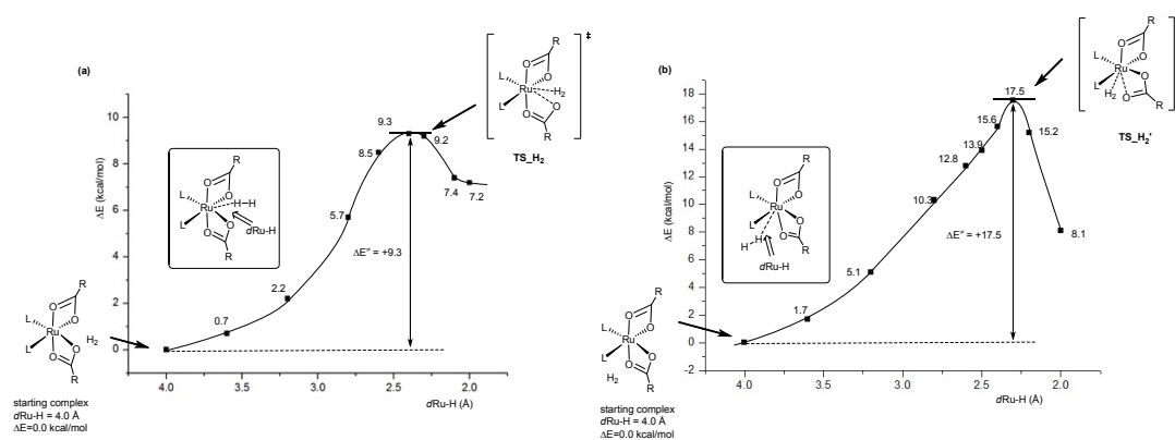
Figure S4. Estimated energy barriers for the H 2 coordination of II .
