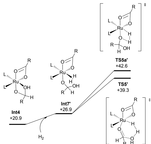
Figure S5. Energy profiles of H 2 heterolysis from Int4 . Gibbs free energies (kcal/mol) are relative to II .
