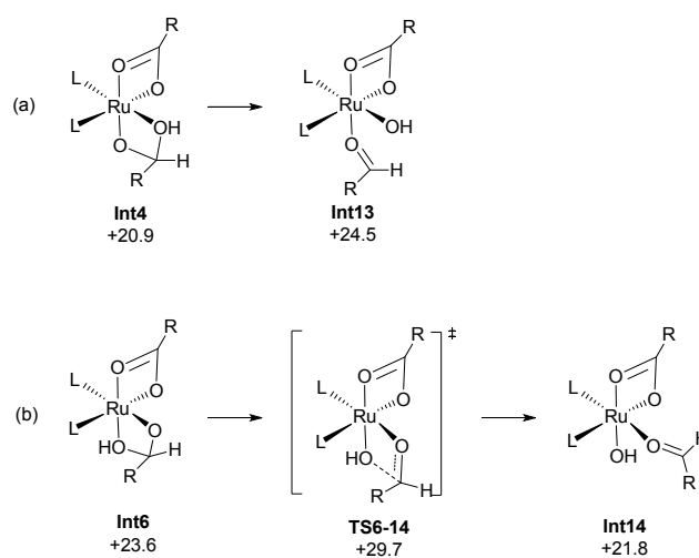
Figure S8. The C-OH bond cleavage of Int4 and Int6 . Gibbs free energies (kcal/mol) are relative to II .
