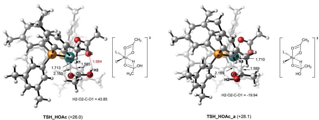
Figure S13. Two types of hydride migration transition states of HOAc. Bond distances and angles are given in [Å] and [°], respectively. Gibbs free energies are relative to (P(3,5\text{-xylyl})_3)_2\text{Ru}(\kappa^2\text{-OAc})_2 .
