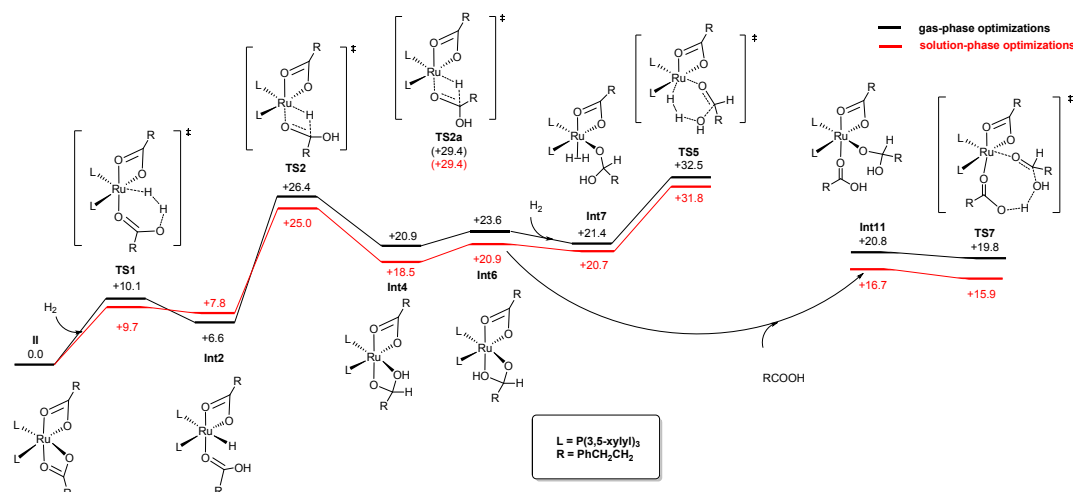
Figure S1. Computational results of gas-phase optimizations (M06/SDD-6-311+G(2d,p)(SMD)//B3LYP/Lan12DZ-6-31G(d) and solution-phase optimizations ( \omega b97X-D/SDD-6-311+G(2d,p)(SMD)// \omega b97X-D/Lan12DZ-6-31G(d)(SMD)
