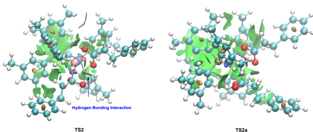
Figure S12. Noncovalent interaction analysis of transition states TS2 and TS2a .
