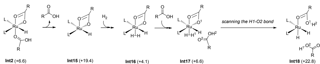
Figure S11. The ionic hydrogenation mechanism
