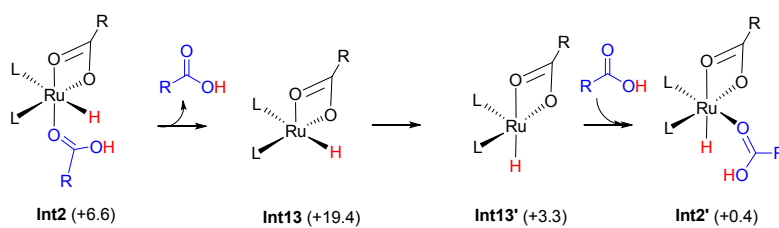
Figure S9. The isomerization of Int2 to Int2' .
