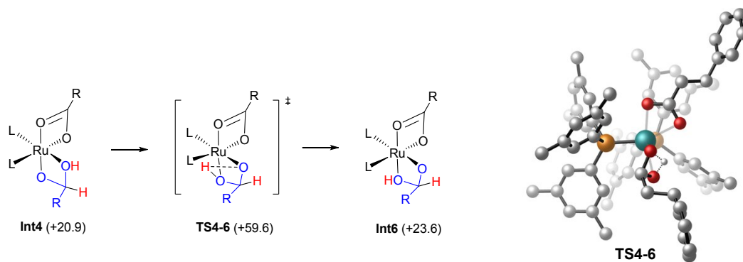
Figure S7. Direct proton transfer of Int4 . Gibbs free energies (kcal/mol) are relative to II .
