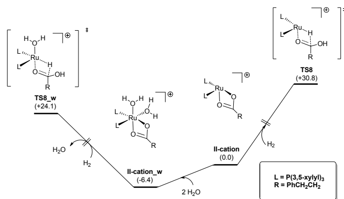
Figure S10. Energy profiles of hydride migration from the cationic Ru complex II-cation . Gibbs free energies are showed in kcal/mol.
