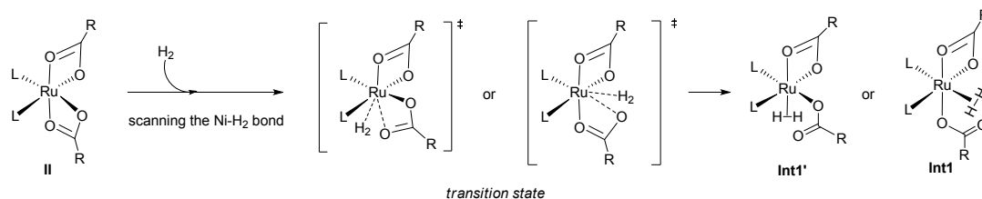
Figure S3. The proposed transition states for H 2 coordination
