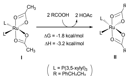
Figure S2. Ligand exchange between I and carboxylic acid.
