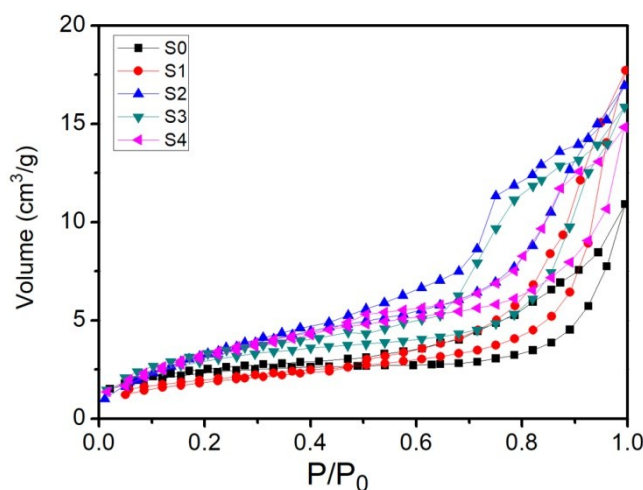
Figure S1 N 2 adsorption-desorption isotherms of S0, S1, S2, S3, and S4 sample.
