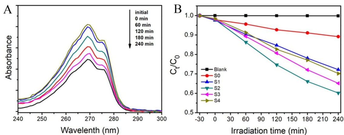
Figure S2 (A) Absorption spectra of phenol solution at different irradiation times in the presence of S2. (B) Photocatalytic degradation ratio of phenol versus irradiation time by using different samples.
