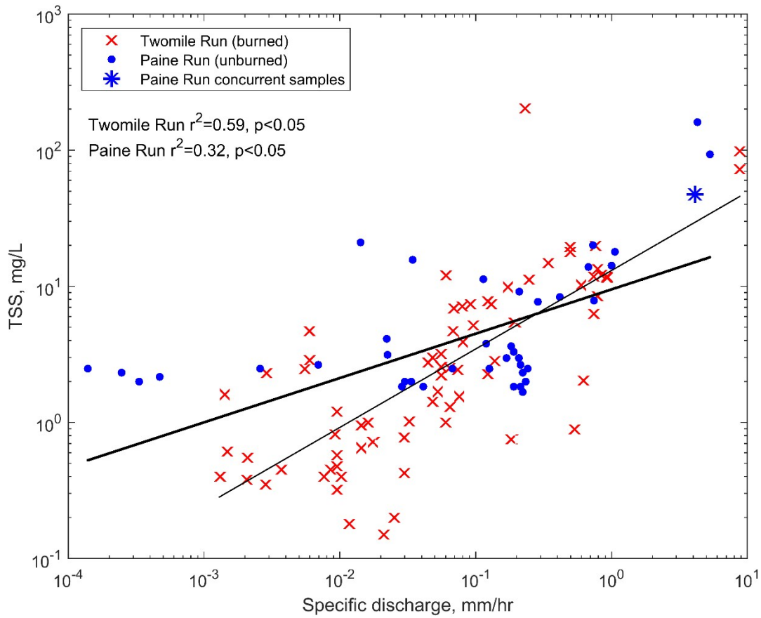
Figure S2. Total Suspended Sediment (TSS) versus specific discharge, and corresponding regression lines, at Twomile Run (thin line) and Paine Run (thick line). The two sites have similar ranges in discharge and TSS.
