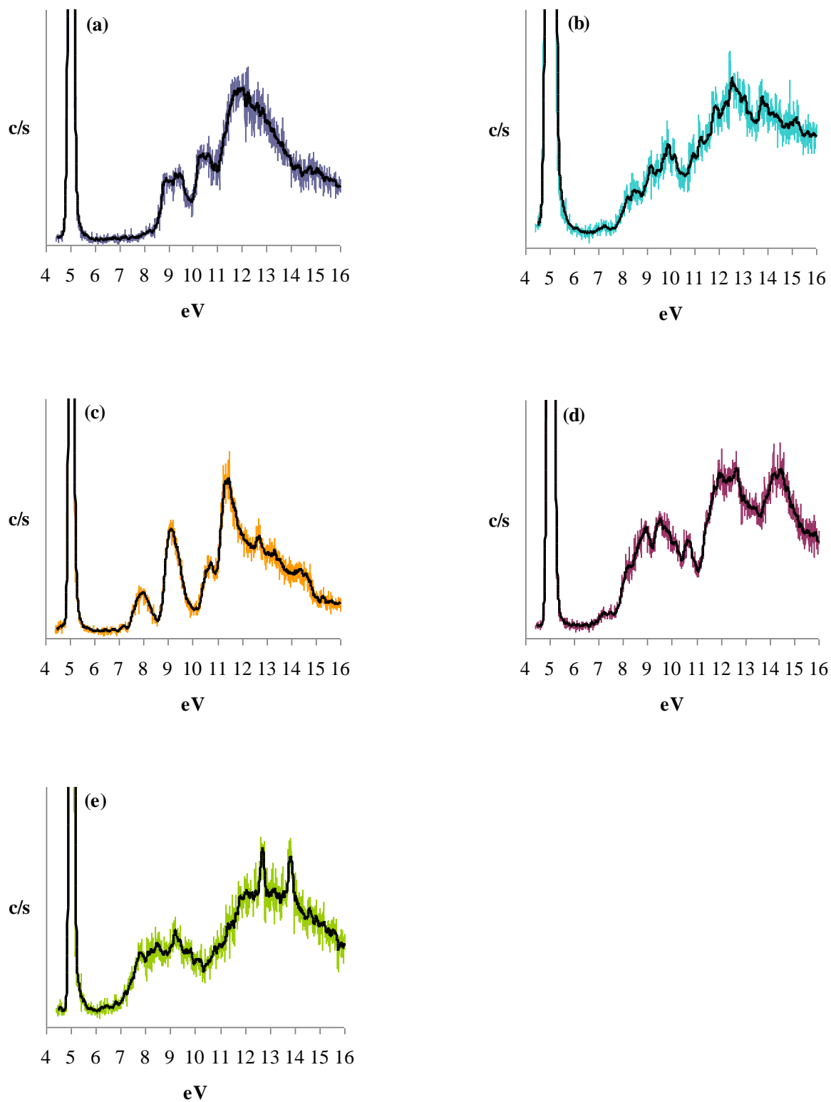
Fig.A. Photoelectronic spectra of (a) OH-IBU; (b) MET; (c) DFC; (d) CBZ; (e) CIP
