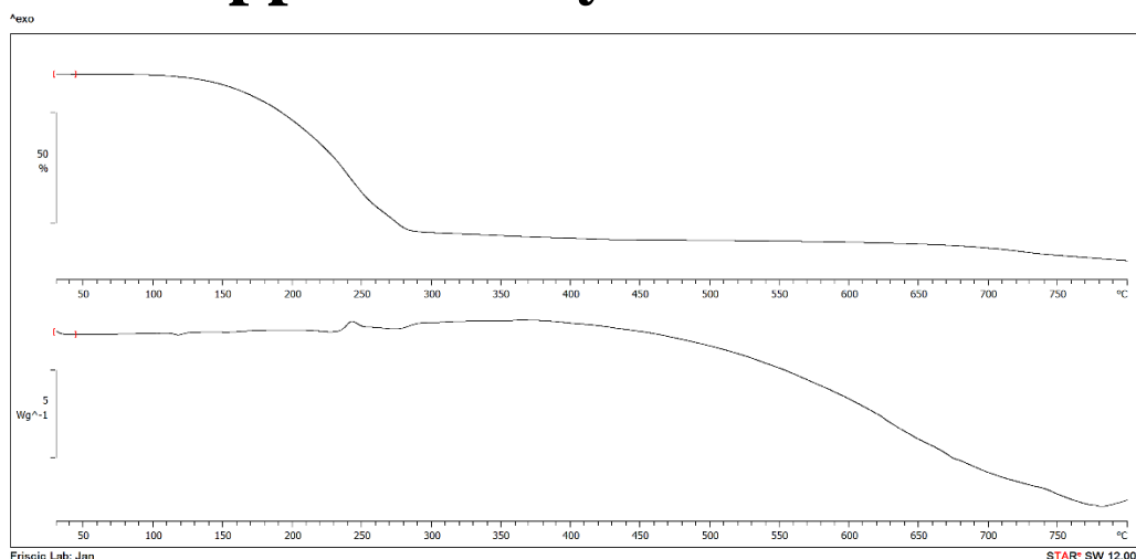
Figure S1. Combined TGA (top) and DSC (bottom) thermograms for 1 , recorded in a dynamic atmosphere of nitrogen. The initial sample weight was 4.30 mg, and the first thermal weight loss step amounts to ca. 74.7%.
