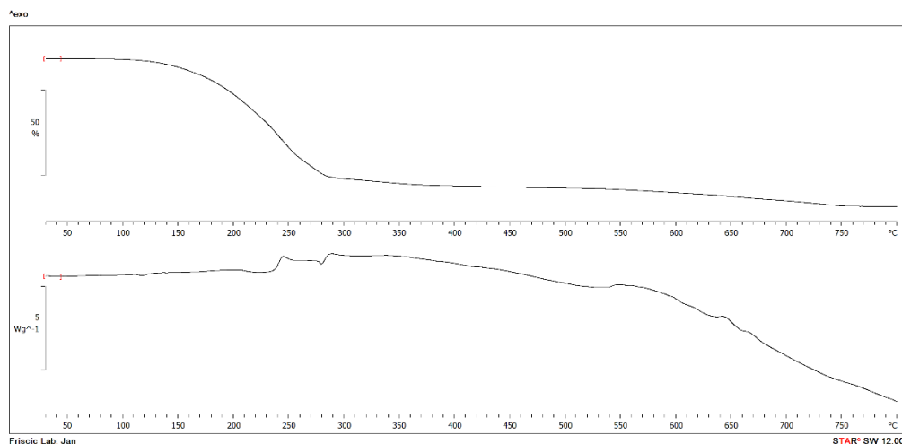
Figure S2. Combined TGA (top) and DSC (bottom) thermograms for 1 , recorded in a dynamic atmosphere of air. The initial sample weight was 4.82 mg, and the first thermal weight loss step amounts to ca. 73.0%.
