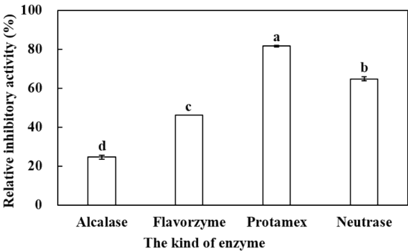
Supplementary Figure S3 Comparative ACE inhibitory activities of sea cucumber gonad hydrolysates by different commercial enzymes with hydrolysis time of 6 h and E/S ratio of 1.0 %.
