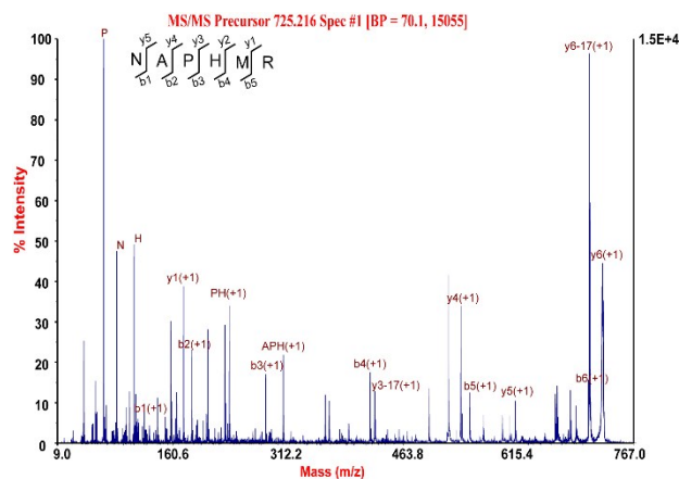
Supplementary Figure S2 The MS/MS spectrum of synthetic peptide NAPHMR.
