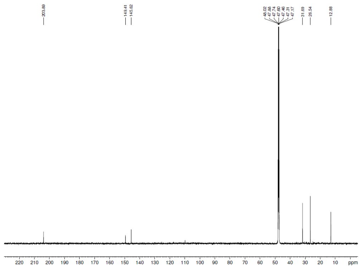
Fig. S2 ^{13}\text{C} NMR spectrum of compound 1
