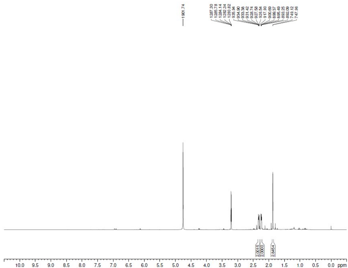
Fig. S1 ^1\text{H} NMR spectrum of compound 1
