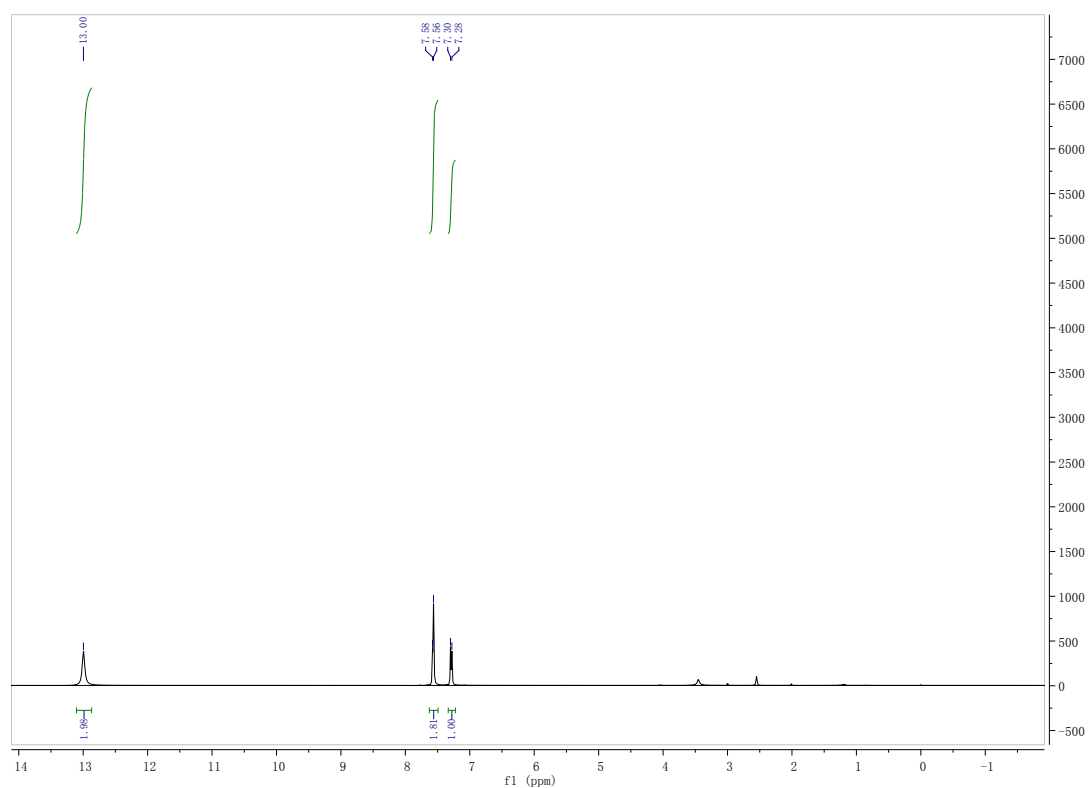
13 C NMR spectrum of compound 3w
