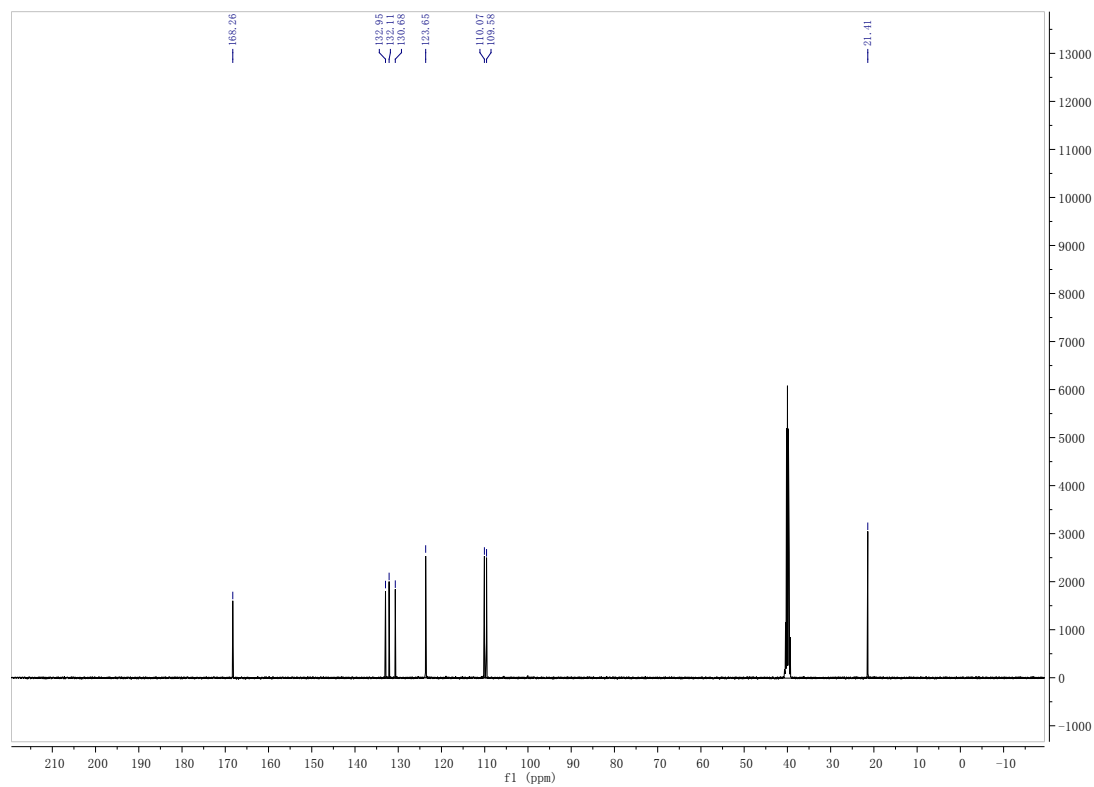
^{13}\text{C} NMR spectrum of compound 3y
