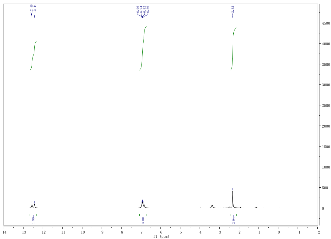
13 C NMR spectrum of compound 3za
