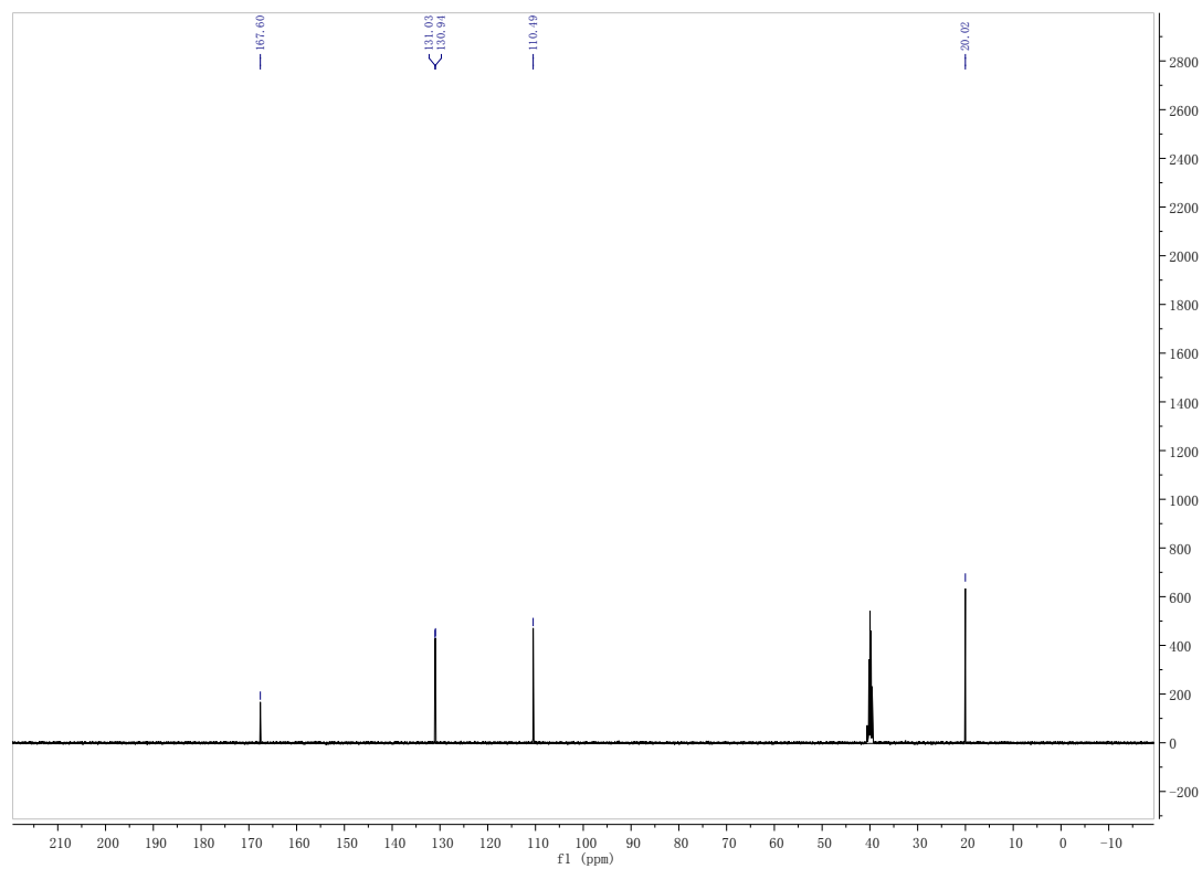
13 C NMR spectrum of compound 3z
