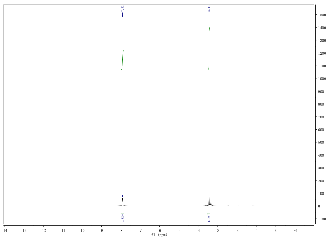
^{13}\text{C} NMR spectrum of compound 3zc
