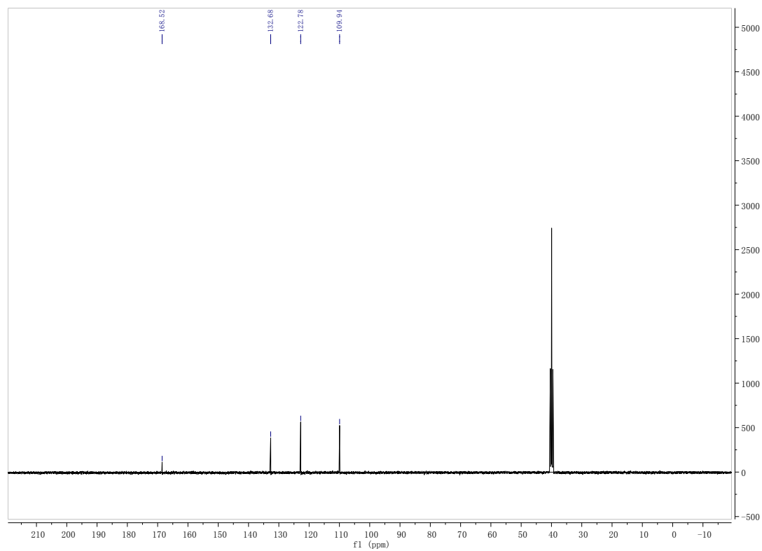
13 C NMR spectrum of compound 3q
