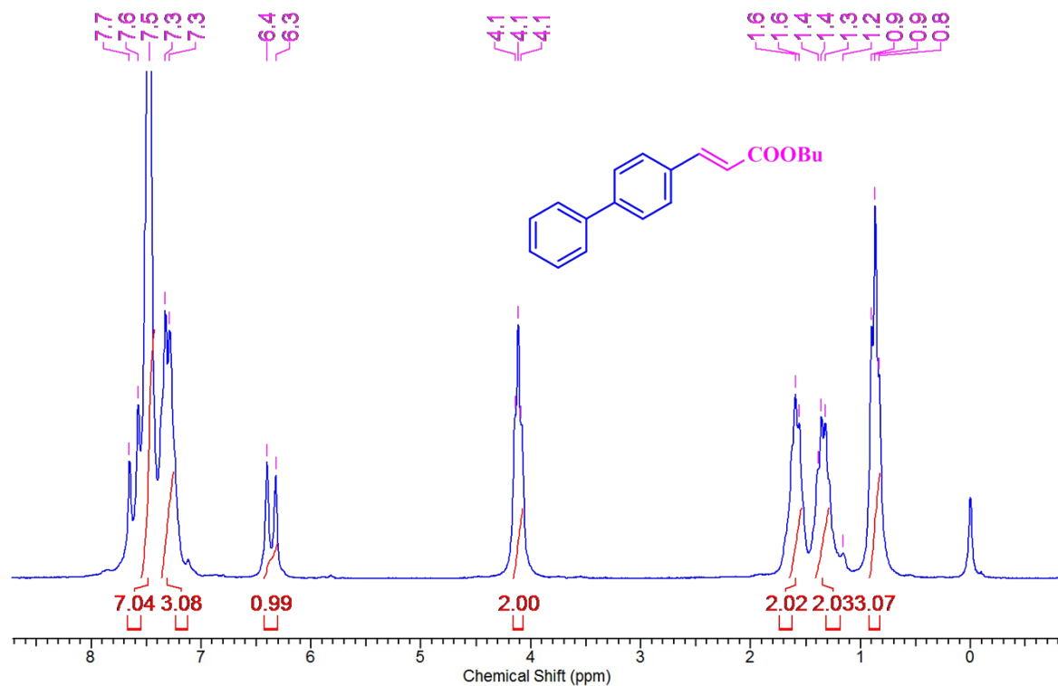
13 C NMR spectrum of butyl( E )-3-([1,1'-biphenyl]-4-yl)acrylate (Table 4, entry 26):
