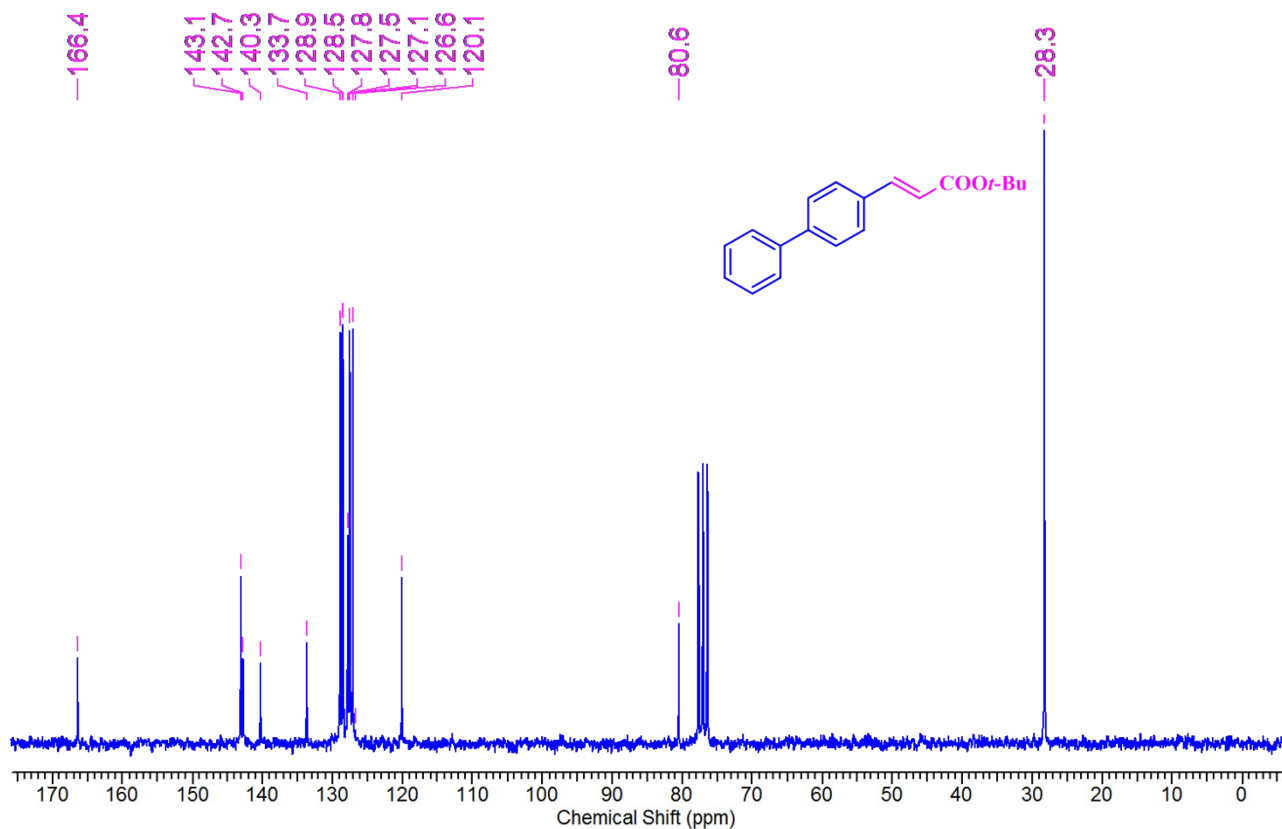
1 H NMR spectrum of butyl( E )-3-([1,1'-biphenyl]-4-yl)acrylate (Table 4, entry 26):
