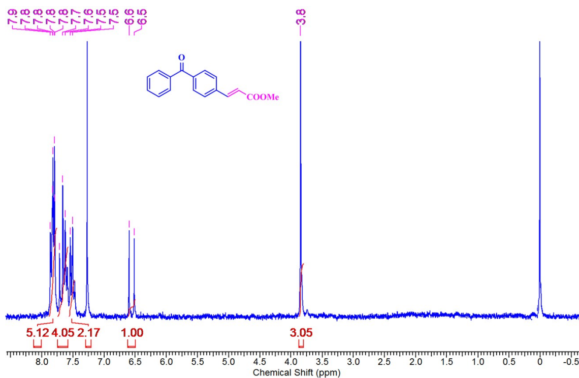
13 C NMR spectrum of methyl( E )-3-(4-benzoylphenyl)acrylate (Table 4, entry 32):
