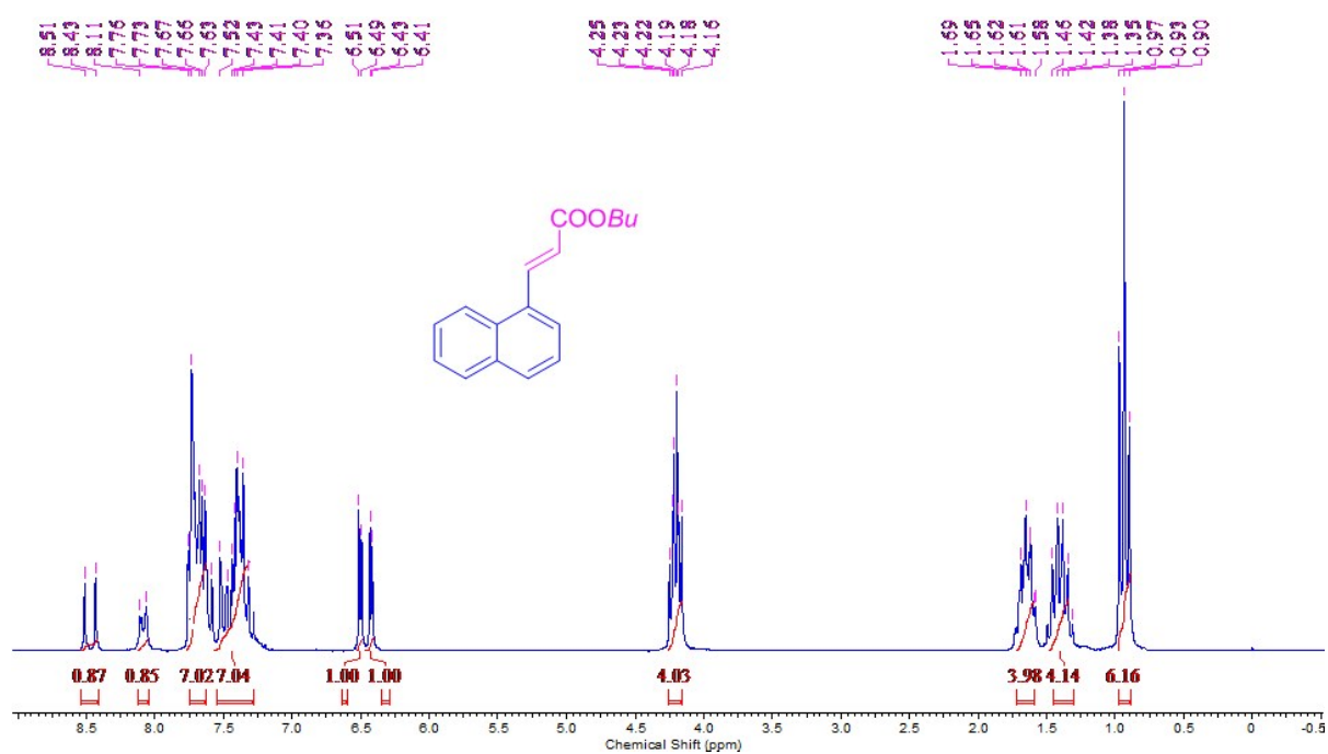
13 C NMR spectrum of butyl( E )-3-(naphthalen-1-yl)acrylate (Table 4, entry 34):
