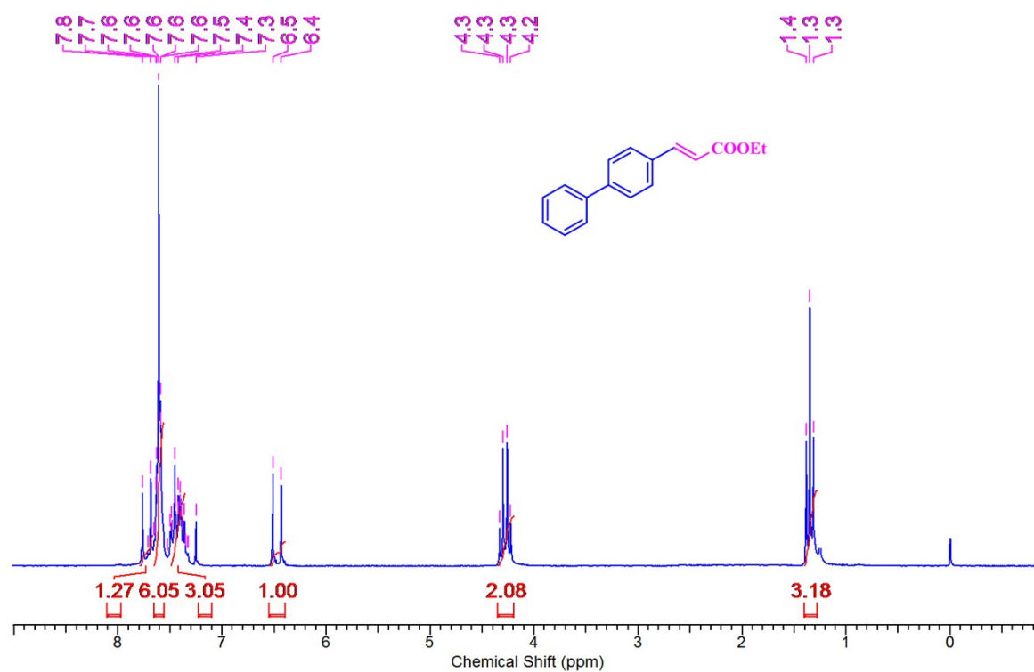
13 C NMR spectrum of ethyl( E )-3-([1,1'-biphenyl]-4-yl)acrylate (Table 4, entry 27):
