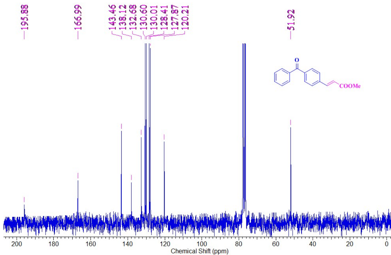
1 H NMR spectrum of tert-butyl( E )-3-(naphthalen-1-yl)acrylate (Table 4, entry 33):
