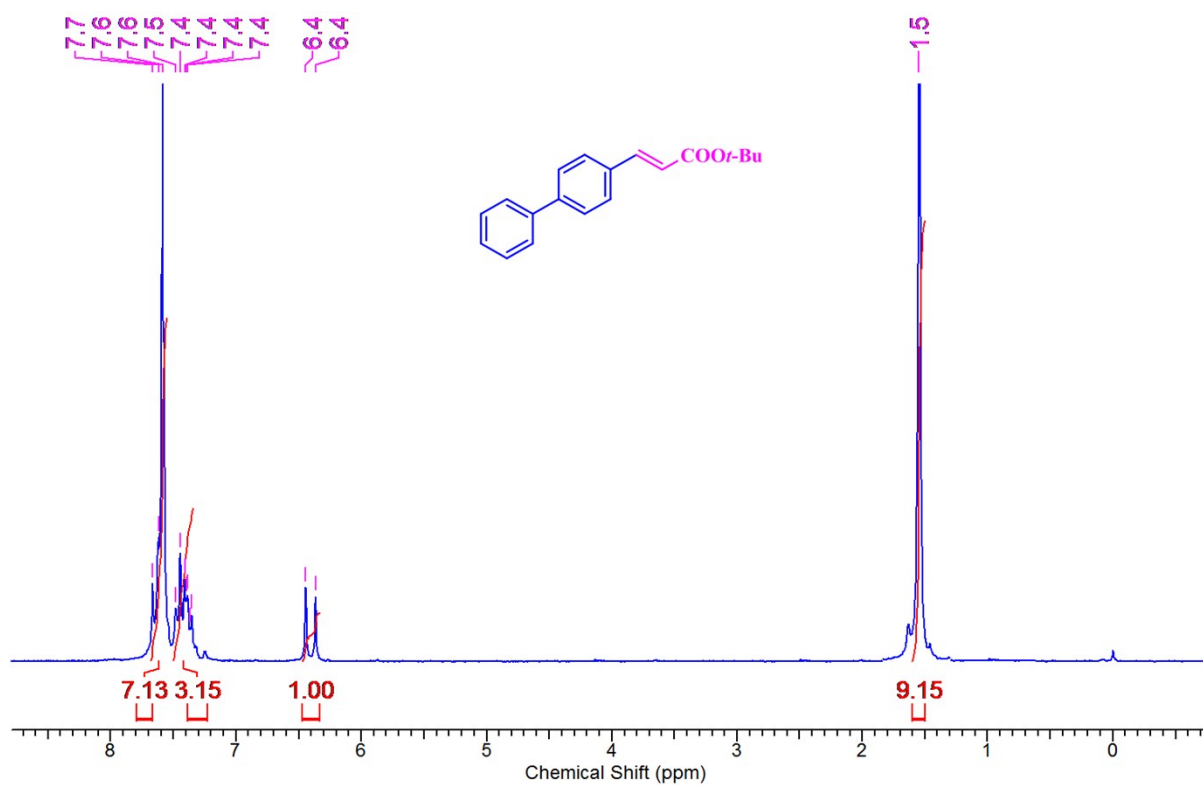
13 C NMR spectrum of tert-butyl( E )-3-([1,1'-biphenyl]-4-yl)acrylate (Table 4, entry 25):
